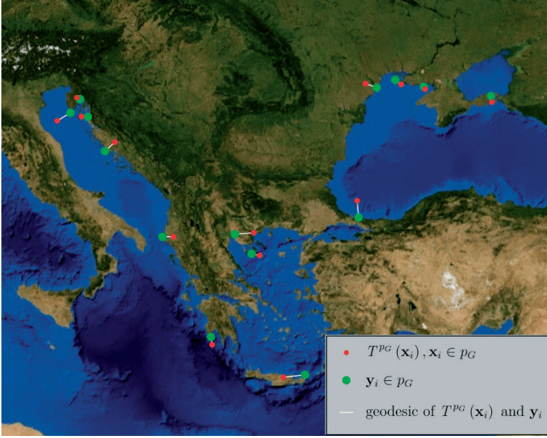
FIGURE 2.4. Optimal local affine transformation T^{p_G} obtained by using the corresponding points set p_G = p_1 \cup p_2 \cup p_3 . The image shows the transformed points from the Strabo's map in red and their corresponding points in WGS in green. One can see that all the points are transformed relatively closely. However, in the previous local transformations, see Figures 2.1–2.3, the points from the sets used for finding the optimal local affine transformations were transformed more accurately, see also Tables 2.1–2.3.
