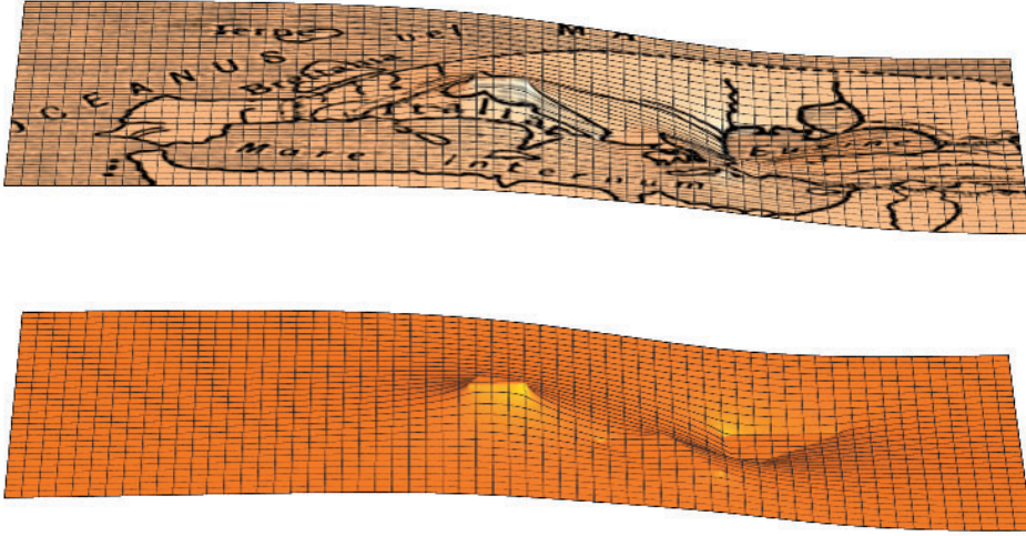
FIGURE 2.7. The images show one of the transformation parameters computed by the LAGL method presented in Figure 2.6. The upper image is plotted with the texture of the Strabo's map of the World , the lower image is plotted without the texture emphasizing the smooth transition of locally optimal affine transformations.
