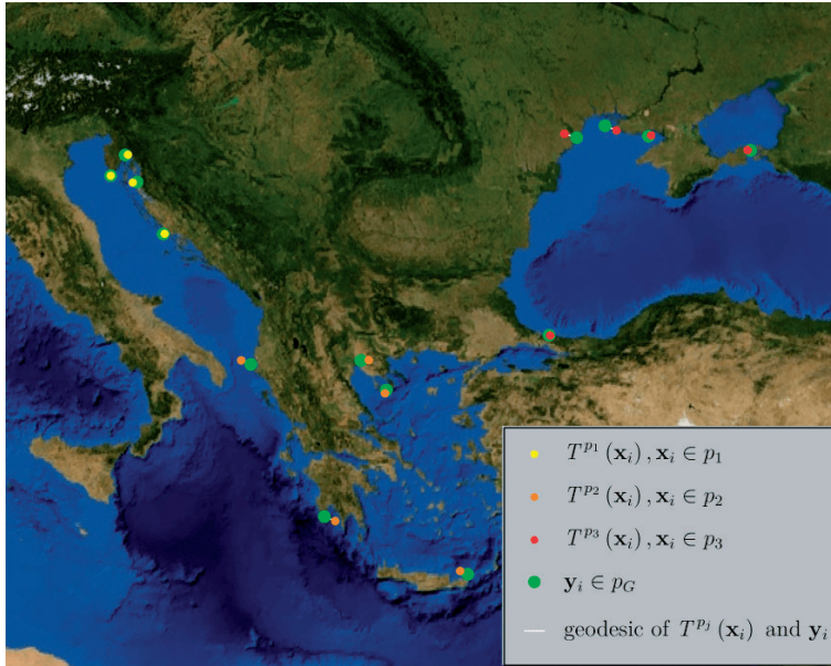
FIGURE 2.6. Transformation found by using the LAGL method. The image illustrates the result for the corresponding points sets p_1 , p_2 and p_3 which are transformed as accurately as by their locally optimal affine transformations T^{p_1} , T^{p_2} and T^{p_3} , see Figures 2.1–2.3.
