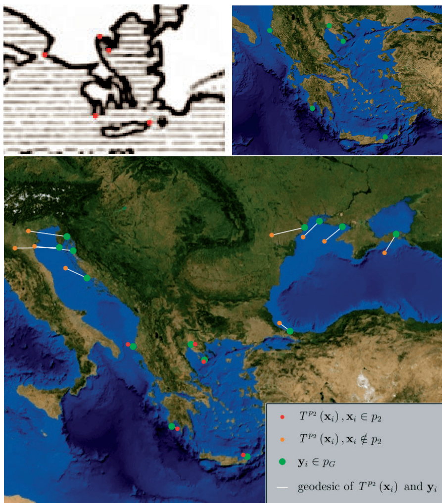
FIGURE 2.2. Optimal local affine transformation T^{p_2} obtained by using the corresponding points set p_2 given in the Greece and Albania region. Top images show the corresponding points, on the left in red on the Strabo's map and on the right in green on the map in WGS. The bottom image shows the transformed points of the set p_2 in red, the transformed points of the sets p_1 and p_3 in orange and their corresponding points in WGS in green. One can see that points in the Greece and Albania region are transformed accurately while the points in other regions are distant from their corresponding points, see also the second rows of Tables 2.1–2.2.
