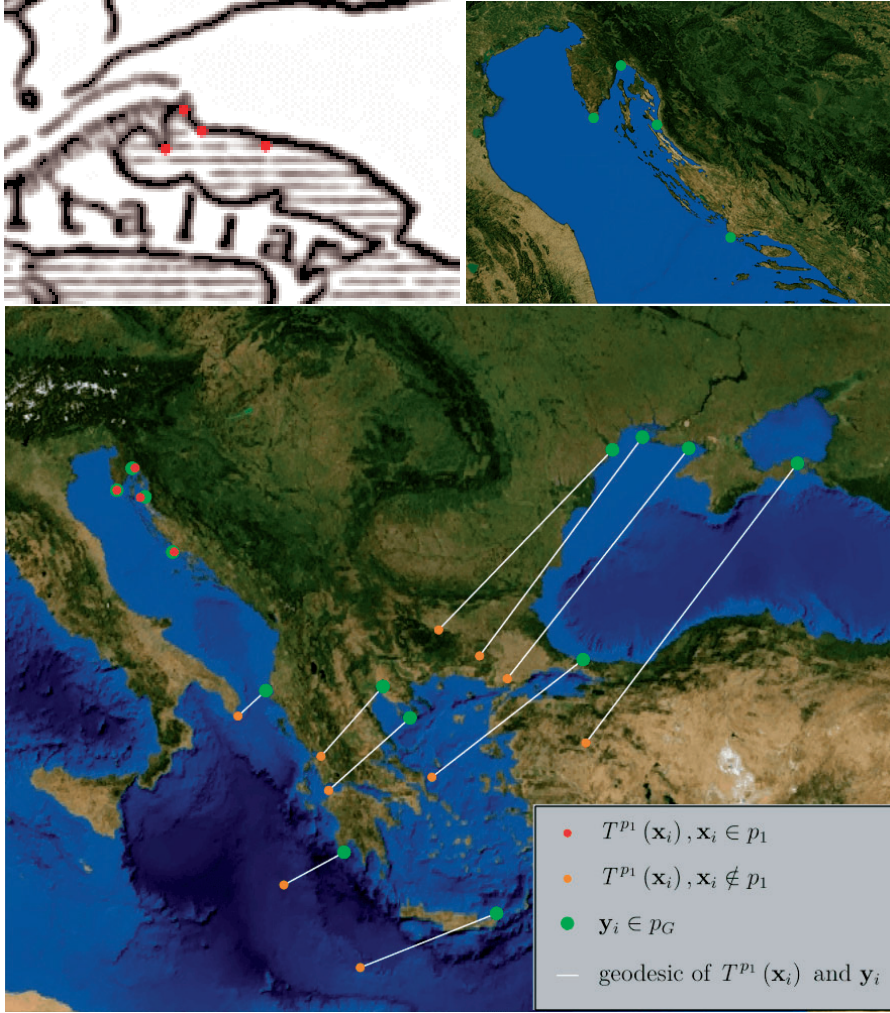
FIGURE 2.1. Optimal local affine transformation T^{p_1} obtained by using the corresponding points set p_1 given on the Adriatic coast. Top images show the corresponding points, on the left in red on the Strabo's map and on the right in green on the map in WGS. The bottom image shows the transformed points of the set p_1 in red, the transformed points of the sets p_2 and p_3 in orange and their corresponding points in WGS in green. One can see that points on Adriatic coast are transformed accurately while the points in other regions are distant from their corresponding points, see also the first rows of Tables 2.1–2.2.
