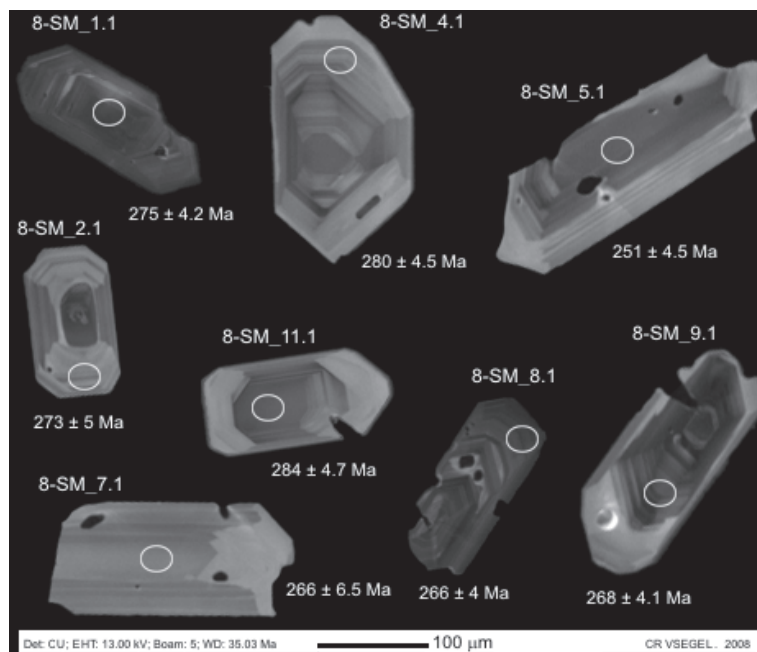
Fig. 4. Selected CL zircon images from the Rožňava Formation 1 st horizon metavolcanites (sample no. 8-SM) and age data based on ^{206}\text{Pb}/^{238}\text{U} ratios with indication of measurement points.
