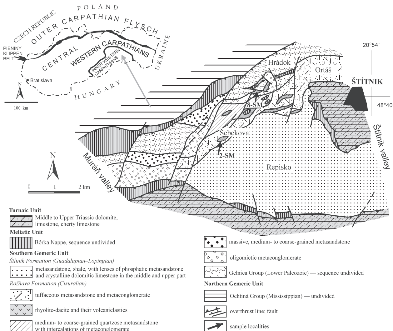
Fig. 1. Geological scheme of the Štítník-Jelšava area with localization of samples (modified after Bajanik et al. 1984 and Mello et al. 1996).
