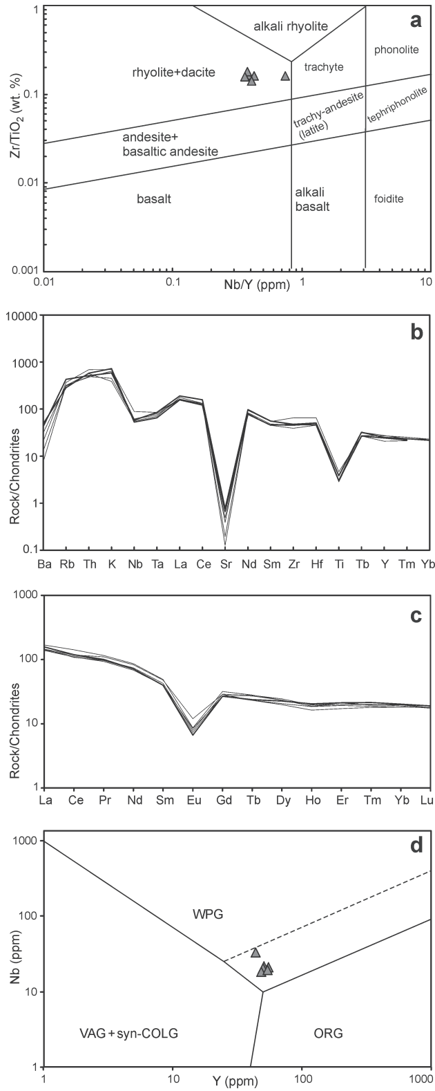
Fig. 3. Rožnava Formation acid volcanite characteristics based on the chemical composition. a — Zr/TiO 2 (wt. %) vs. Nb/Y (ppm) diagram after Winchester & Floyd (1977) modified by Pearce (1996). b — Chondrite normalized (Thompson 1982) trace elements abundances. c — Chondrite normalized REE patterns. Normalizing values are after Taylor & McLennan (1985). d — Variation Nb (ppm) vs. Y (ppm) with indication of tectonic settings after Pearce et al. (1984).
