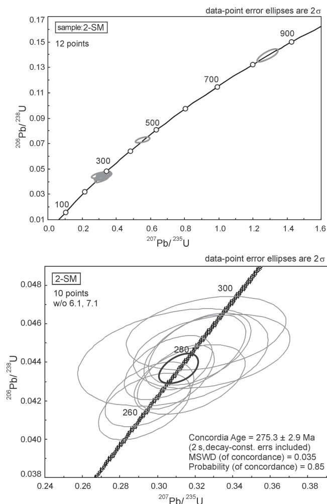
Fig. 7. Concordia diagrams of zircon age data from the Rožňava Formation 2 nd horizon metavolcanites (sample no. 2-SM).
