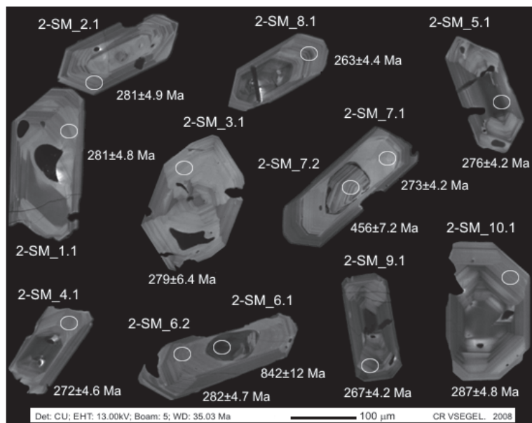
Fig. 6. Selected CL zircon images from the Rožňava Formation 2 nd horizon (sample no. 2-SM) metavolcanites and age data based on ^{206}\text{Pb}/^{238}\text{U} ratios with indication of measurement points.
