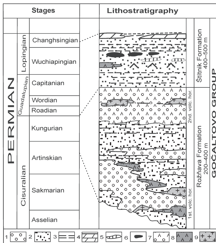
Fig. 2. Gočaltovo Group lithostratigraphic scheme (modified after Vozárová & Vozár 1988). Explanation: 1 — metaconglomerate; 2 — metasandstone; 3 — shale; 4 — crystalline dolomitic limestone; 5 — albitolite; 6 — phosphatic metasandstone; 7 — tuffaceous/sedimentary mixed rocks; 8 — rhyolite-dacite volcanoclastics; 9 — rhyolite-dacite.
