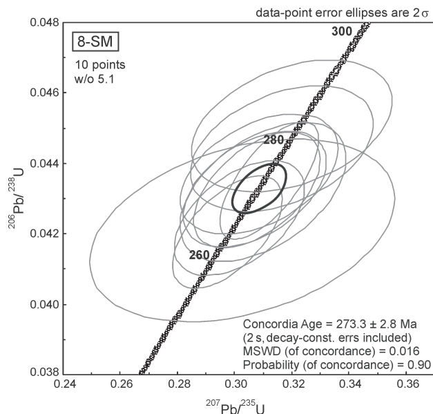
Fig. 5. Rožňava Formation 1 st horizon metavolcanites concordia diagram of zircon age data (sample no. 8-SM).
