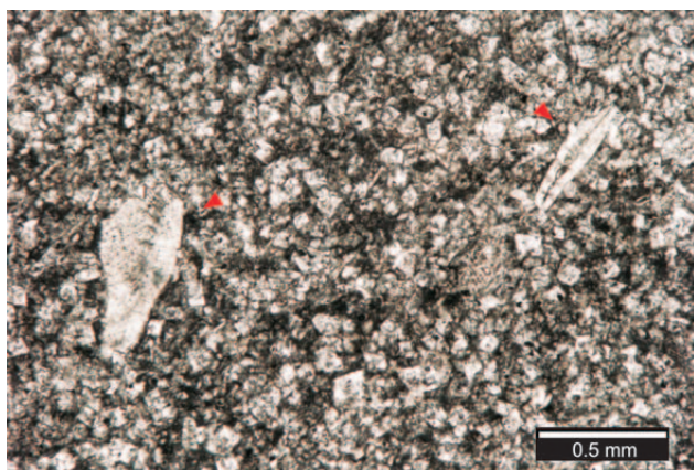
Fig. 10. Microphotograph of intensively dolomitized limestone containing hyaline foraminifer Goupillaudina sp., with frequent subhedral and euhedral dolomite crystals (Sample S-12.2).
