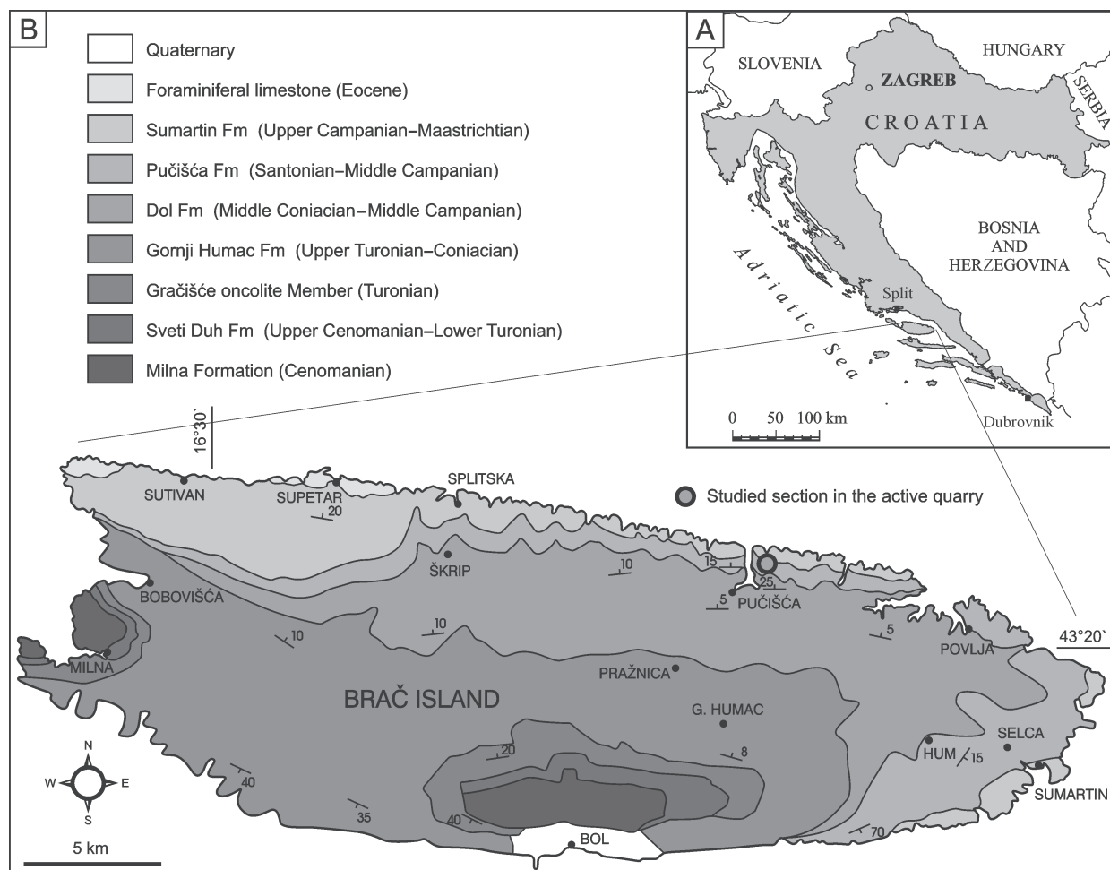
Fig. 1. A — Map showing location of the island of Brač in the eastern Adriatic region. B — Simplified lithostratigraphic map of the island of Brač (modified after Gušić & Jelaska 1990; Steuber et al. 2005) showing the position of the studied section near Pučišća.
