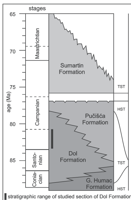
Fig. 2. Chronostratigraphy of the island of Brač with sequence stratigraphic interpretation (adapted from Cvetko Tešović et al. 2001, and Steuber et al. 2005).
