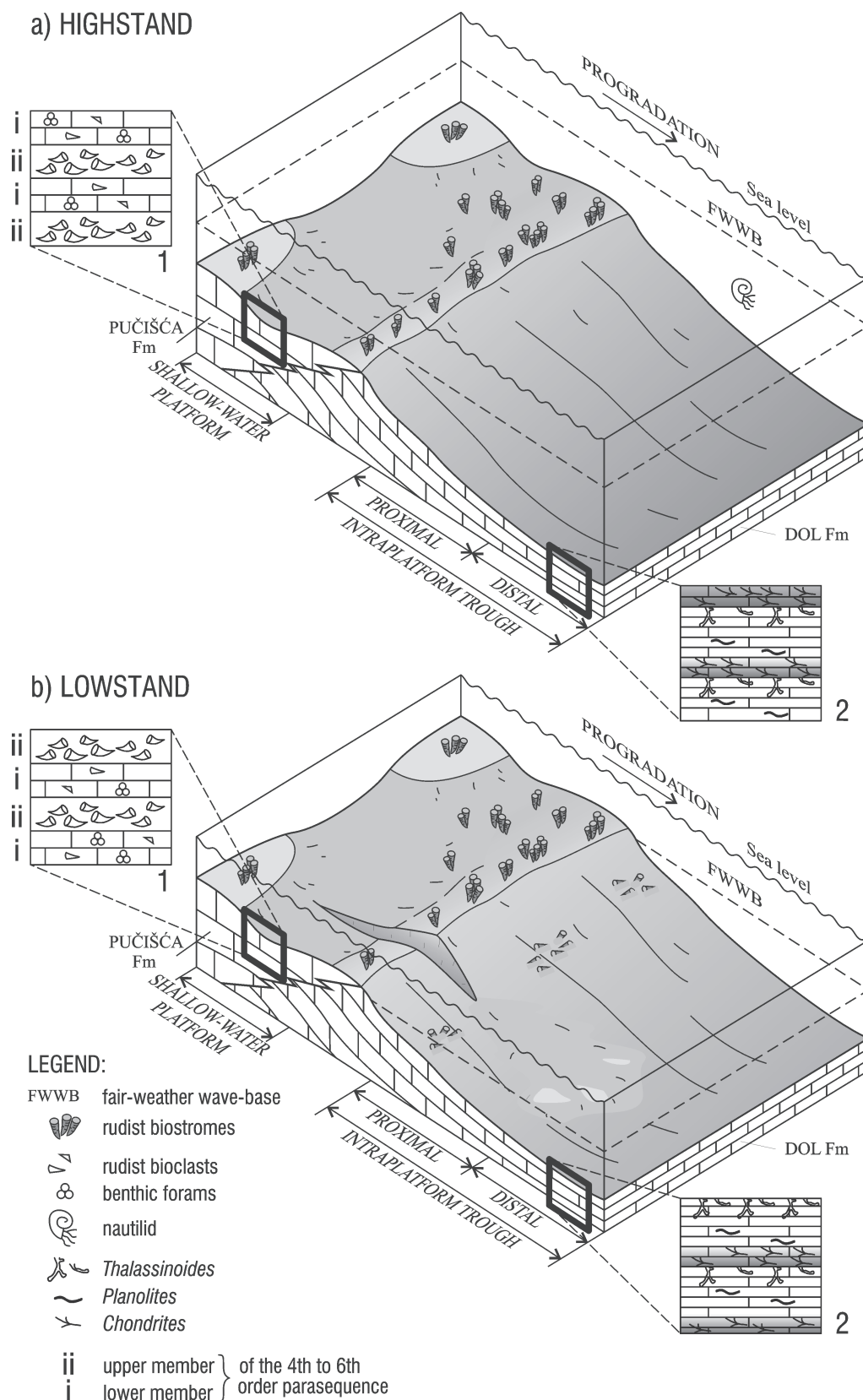
Fig. 11. Schematic reconstructions show the platform margin-slope-basin relationships. a — during high-frequency sea-level highstands when the sea-bottom on the platform margin was positioned below the fair-weather wave-base; b — during high-frequency sea-level lowstands, when the sea-bottom on the platform margin was positioned closer and/or above the fair-weather wave-base (11a.1 and 11b.1 parasequences modified after Moro et al. 2002) (not to scale).
