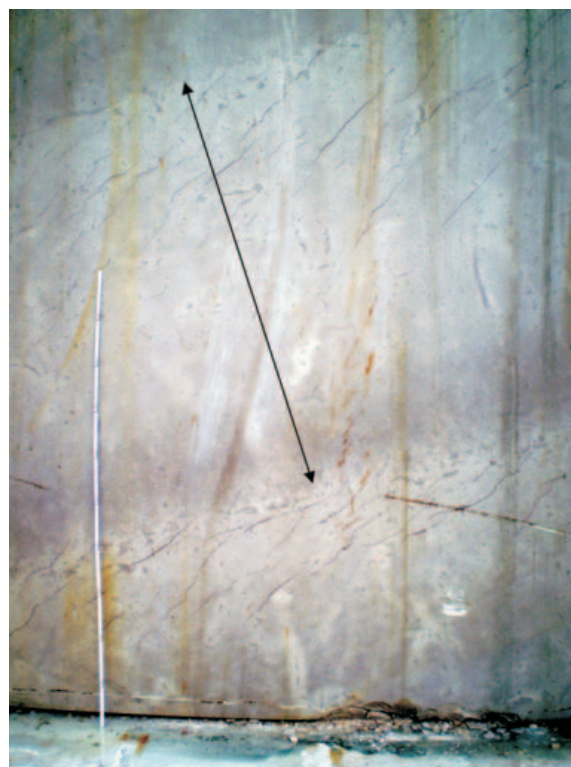
Fig. 5. An individual bed (bed 5) showing dark, completely bioturbated lower part and sparse burrows in the middle and upper parts (scale bar is 1 meter long).
