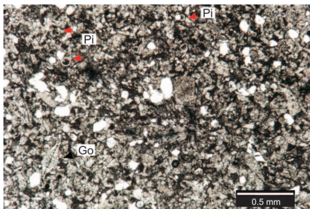
Fig. 8. Microphotograph of bioclastic packstone microfacies with pithonellas (Pi), Goupillaudina sp. (Go) and undefined calcitic debris. Subhedral and euhedral dolomite crystals are frequent (Sample S-4.1).
