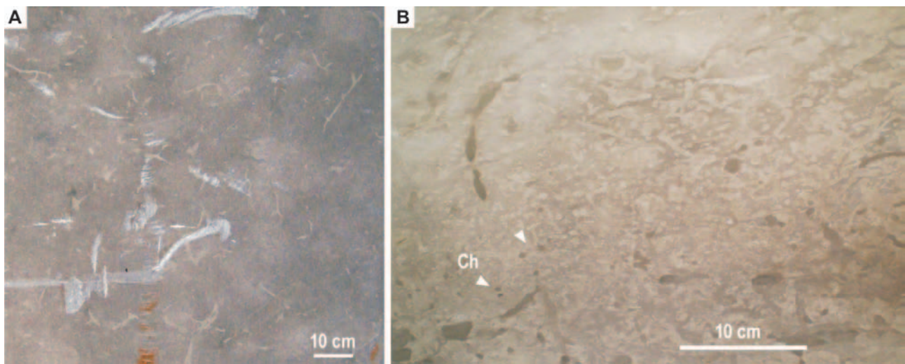
Fig. 6. Trace fossils on vertical surface of the quarry pit: distribution of trace fossils within the lower part of an individual bed built up of dark grey limestone: A — Chondrites ; B — almost completely burrowed part with Chondrites (Ch).
