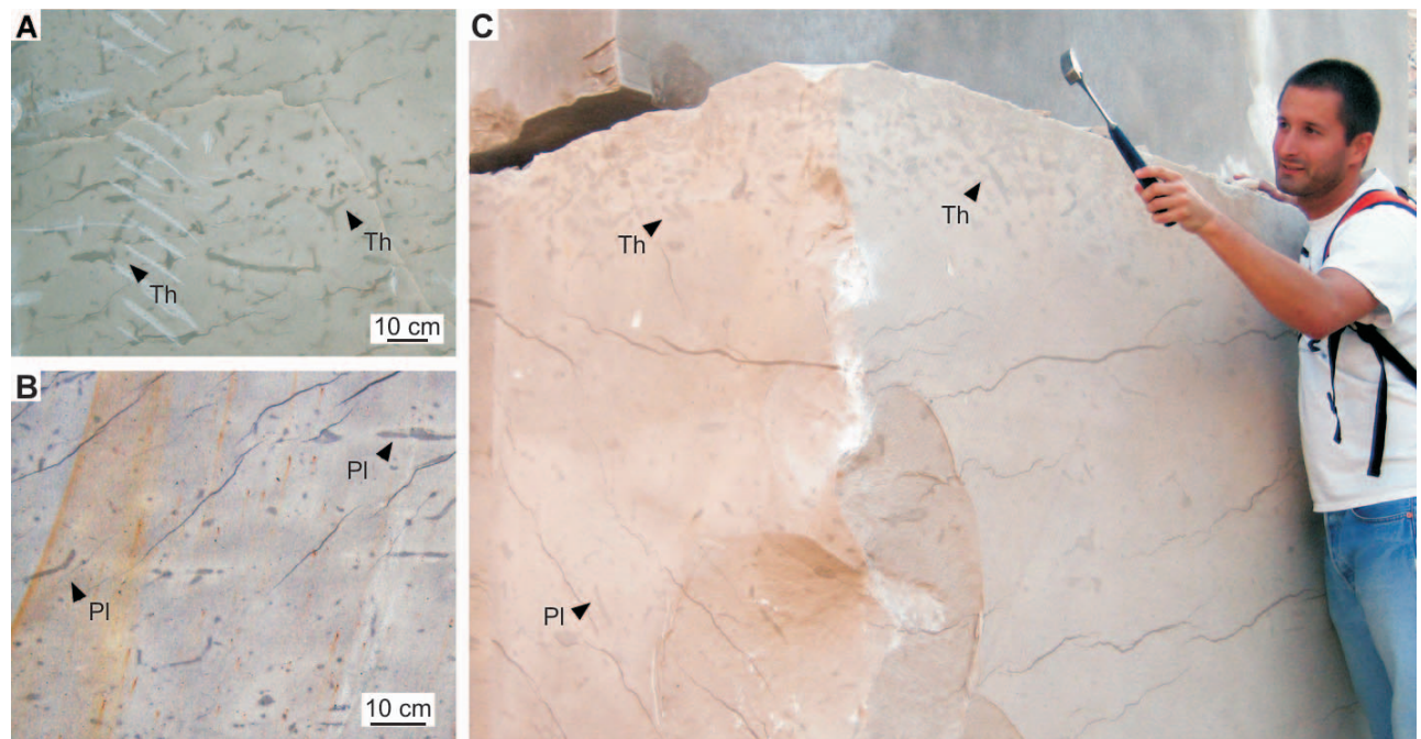
Fig. 7. Trace fossils on vertical surface of the quarry pit: A — Thalassinoides (Th); B — Planolites (Pl); C — distribution of trace fossils within the upper part of an individual bed built up of light grey to white limestone: sparse Planolites (Pl) in the lower part and abundant Thalassinoides (Th) in the upper part.
