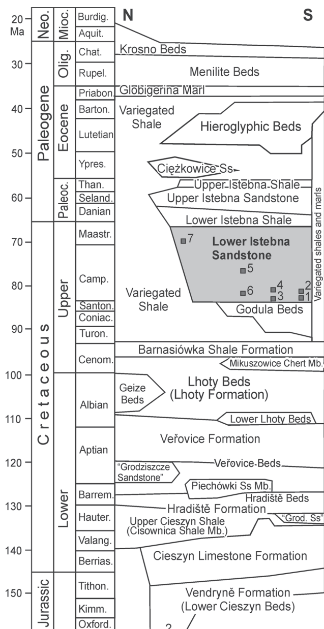
Fig. 2. General stratigraphic scheme of the Cretaceous-Paleocene in the Silesian Nappe (compiled from Oszczytko 2004 and Vašíček et al. 2010, and references therein). The Lower Istebna Beds shaded. Position of the studied outcrops: 1 — Łęki quarry, 2 — Łęki-river and Łęki-klippe sections, 3 — Czaśław 1 quarry, 4 — Czaśław 2 quarry, 5 — Sobolów quarry, 6 — Zonia quarry, 7 — Wola Komborska quarry.
