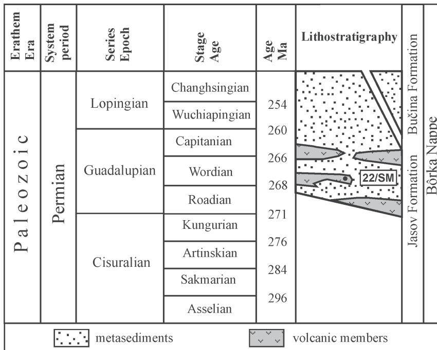
Fig. 4. Bôrka Nappe lithostratigraphic scheme with indication of magmatic zircon samples (modified after Mello et al. 1997, 1998).
