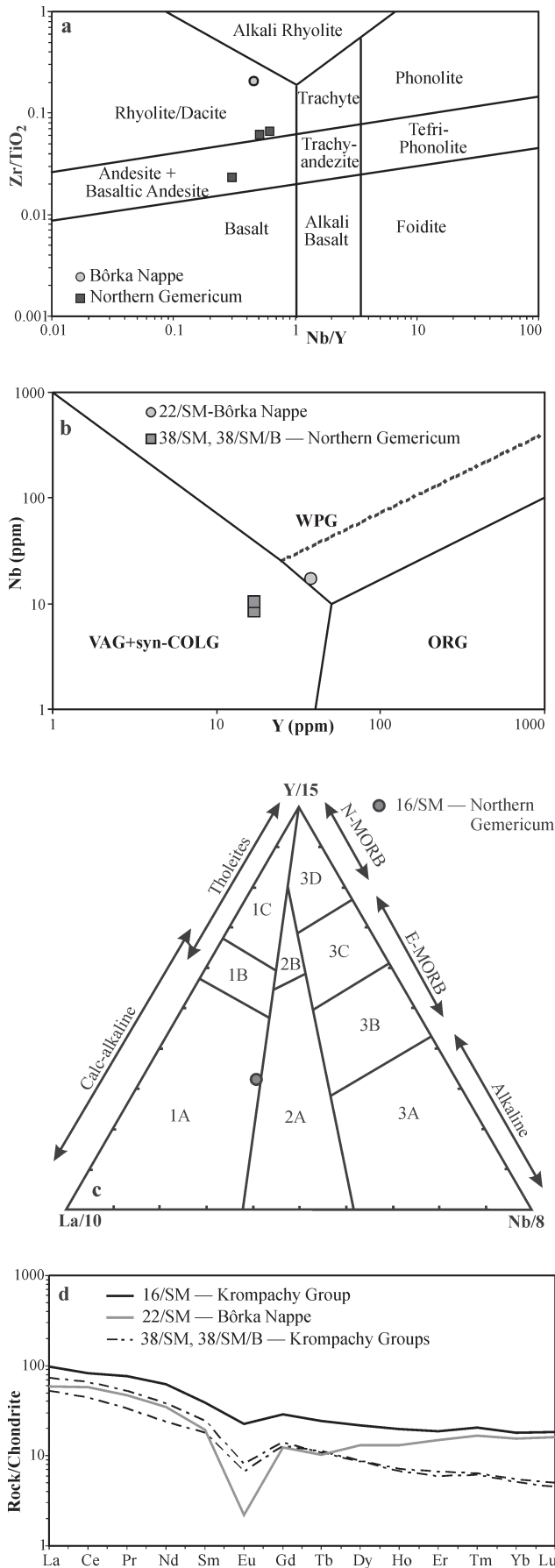
Fig. 3. Northern Gemic and Bôrka Nappe dated volcanite characteristics based on their chemical composition. a — Zr/TiO_2 (wt. %) vs. Nb/Y (ppm) classification diagram after Winchester & Floyd (1977). b — Variations Nb (ppm) vs. Y (ppm) in the acid volcanites with indication of tectonic setting after Pearce et al. (1984); Abbreviations: WPG — within-plate granite, ORG — orogenic granite, VAG + syn-COLG — volcanic arc and syn-collisional granite. c — Position of basaltic andesite (sample no. 16/SM) in the Y/15:La/10:Nb/8 discrimination diagram after (Cabaniš & Leccole 1989); Abbreviations: 1A — calc-alkaline basalts, 1B — calc-alkaline basalts and island-arc tholeiites, 1C — island arc tholeiites, 2A — continental basalts, 2B — back-arc basin basalts, 3A — alkali basalts of within-continental rift, 3B — enriched E-MORB, 3C — slightly enriched E-MORB, 3D — N-MORB. d — Chondrite normalized REE patterns. Normalizing values are after Taylor & McLennan (1985).
