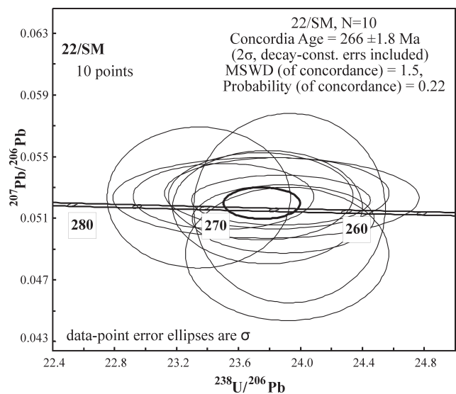
Fig. 7. Concordia diagram of zircon age data from the Bôrka Nappe rhyodacite (sample no. 22/SM).
