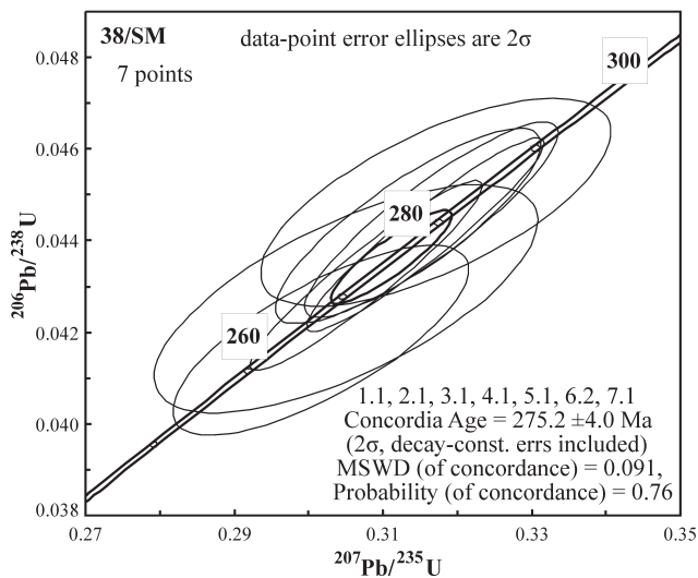
Fig. 5. Concordia diagrams of magmatic zircon ages from the Northern Gemicum rhyodacite (sample no. 38/SM).
