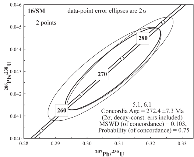
Fig. 6. Concordia diagrams of zircon age data from the Northern Gemic basaltic andesite (sample no. 16/SM).
