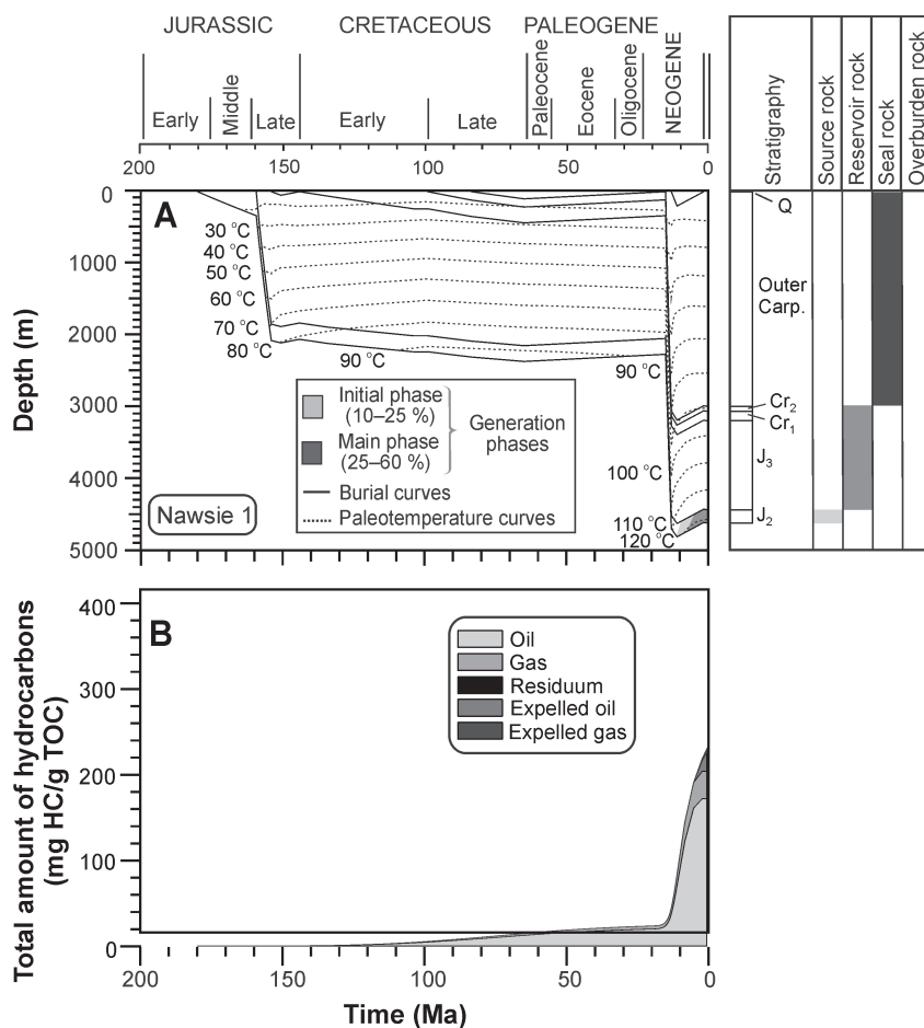
Fig. 6. A — Burial history curves for Jurassic source rocks with generation stages and B — total amount of hydrocarbons generated from the Jurassic source rocks in Nawsie 1 well. For the abbreviations see Fig. 2.
