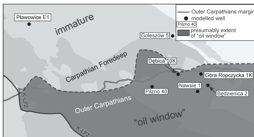
Fig. 4. The presumably extent of the “oil window” in the Jurassic and Cretaceous strata in the Kraków-Rzeszów area.
