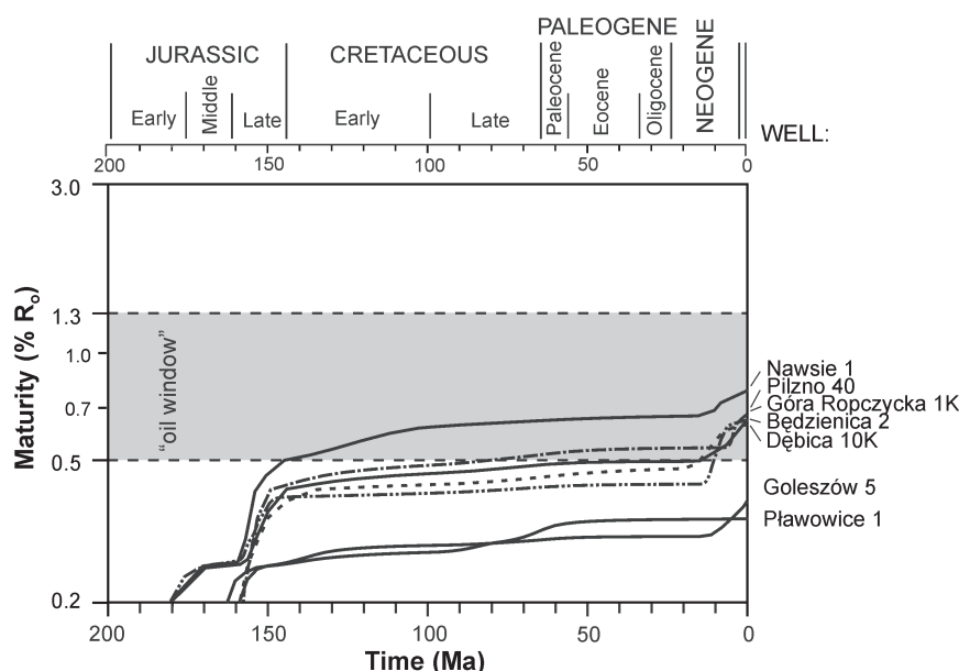
Fig. 3. Maturity evolution curves for the Jurassic source rocks in profiles of analysed wells.
