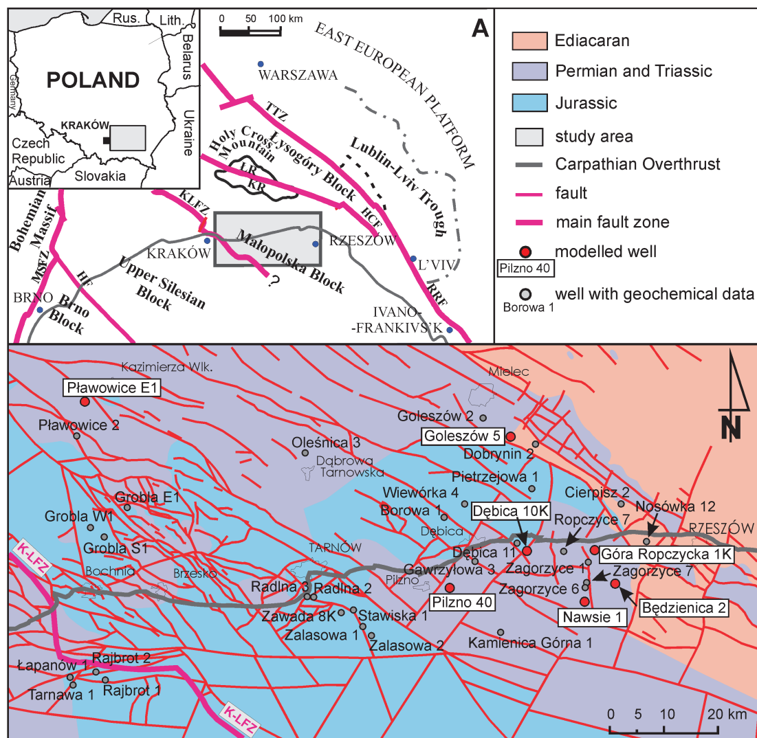
Fig. 1. Extent of the lowermost Mesozoic strata in the study area with location of 1-D modelled wells. Rus. — Russia, Lith. — Lithuania, MSFZ — Moravian-Silesian Fault Zone, HF — Hana Fault, KLFZ — Kraków-Lubliniec Fault Zone, HCF — Holy Cross Fault, RRF — Rava Ruska Fault, TTZ — Teisseyre-Tornquist Zone, LR — Łysogóry Region, KR — Kielce Region.
