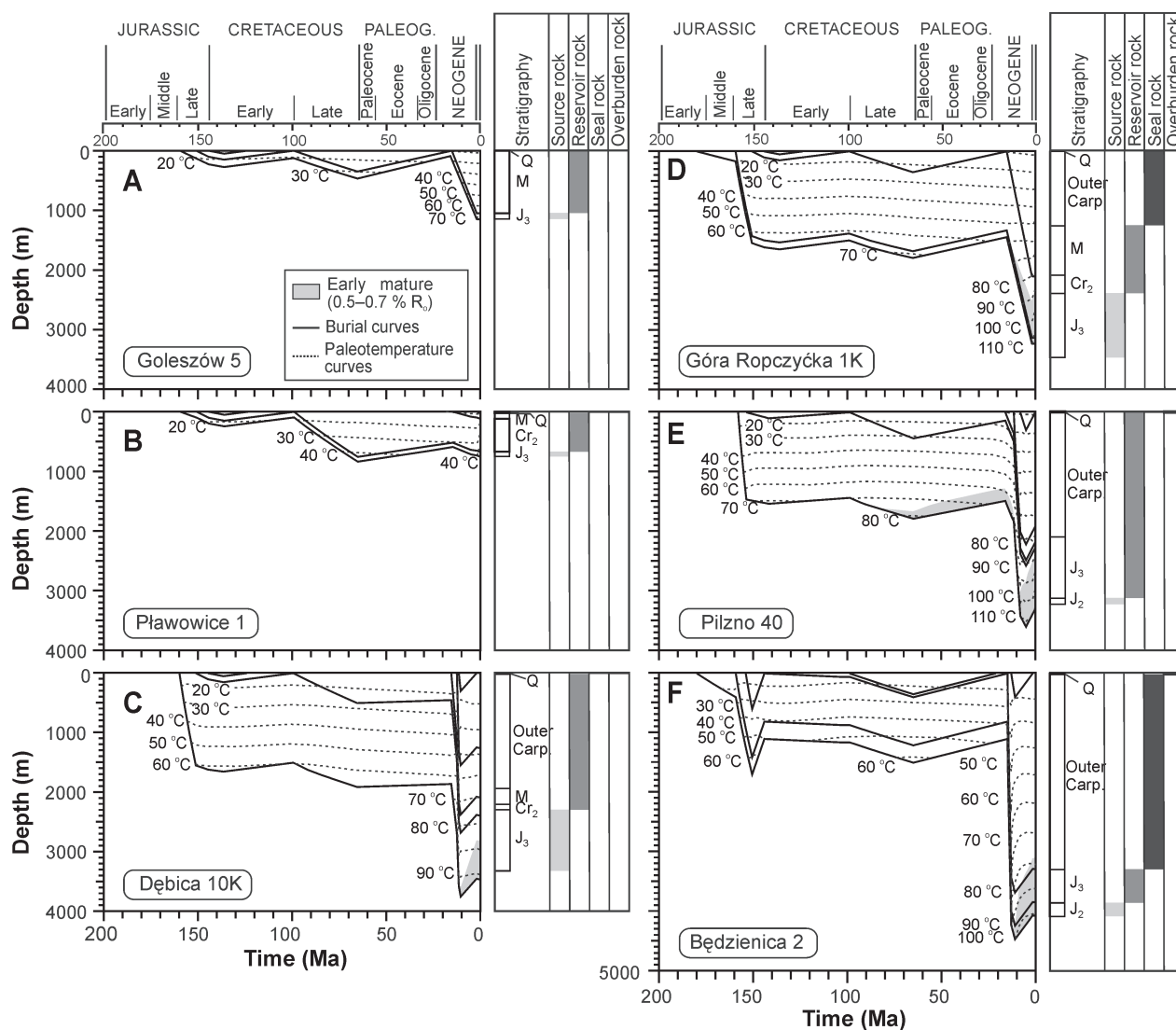
Fig. 2. Burial history curves of the (A) Goleszów 5, (B) Pławowice 1, (C) Dębica 10K, (D) Góra Ropczycka 1 and (E) Pilzno 40 wells and (F) Będzienia 2 wells. J 2 — Middle Jurassic, J 3 — Late Jurassic, Cr 2 — Late Cretaceous, M — Miocene, Outer Carp. — Outer Carpathians, Q — Quaternary.
