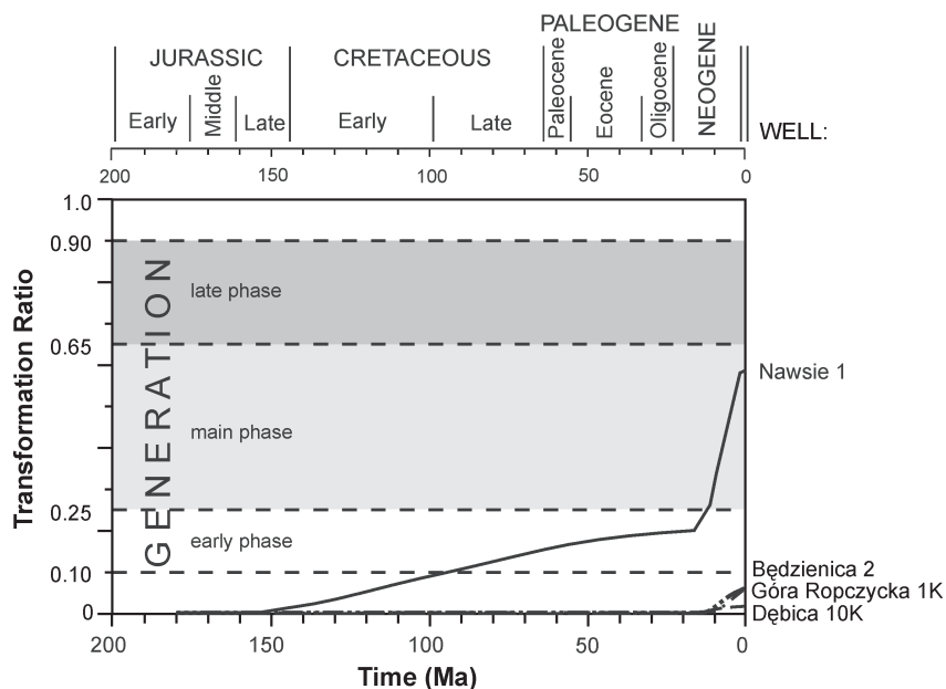
Fig. 5. Transformation ratio of kerogen in the Jurassic source rocks in the profiles of analysed wells.
