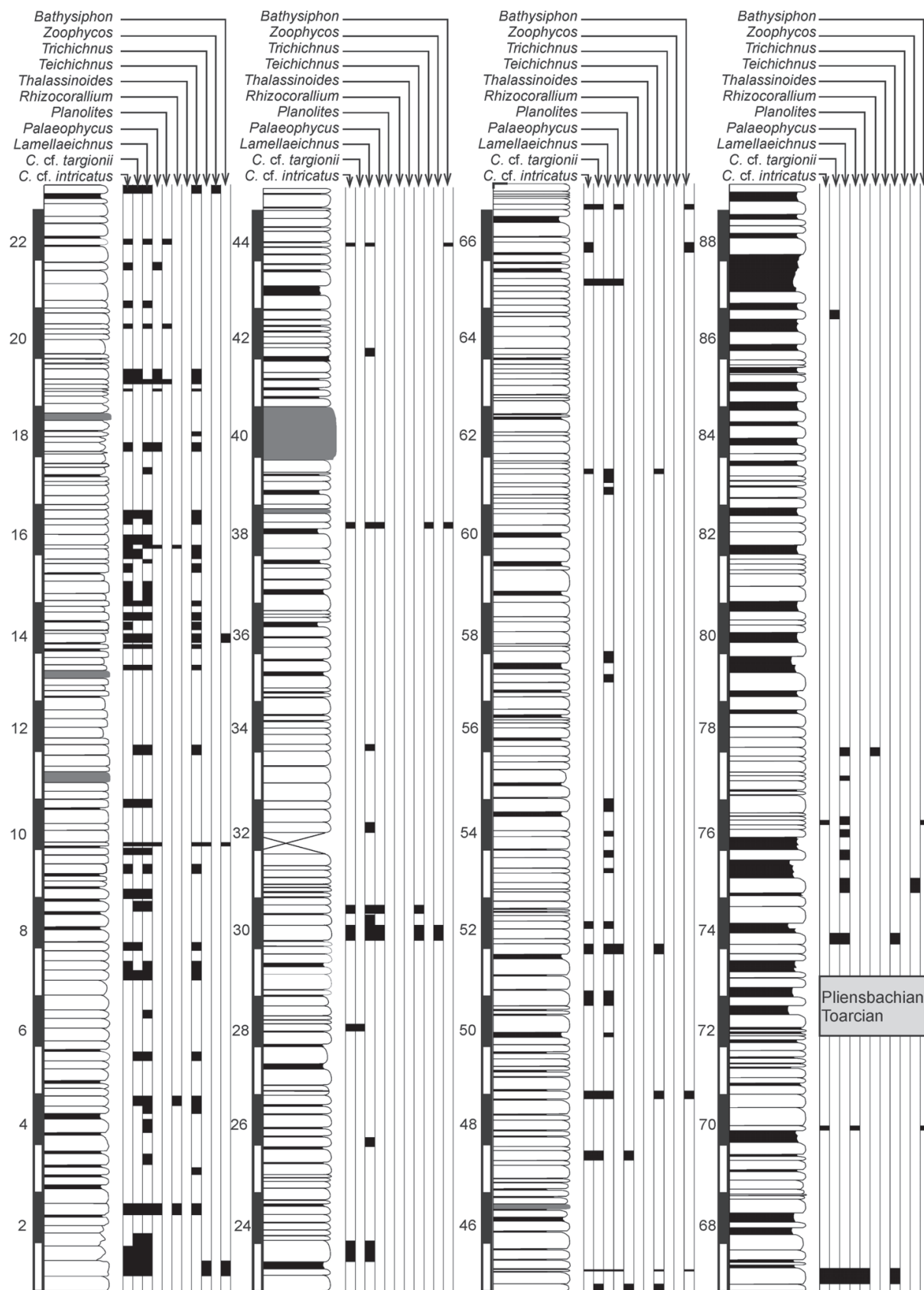
Fig. 3. The stratigraphic distribution of trace fossils and Bathysiphon in the Skladaná Skala section. White beds represent marly limestones, grey beds represent cherty spiculites, and black beds represent marls. The location of the Pliensbachian/Toarcian boundary is approximate and is placed at the boundary between the carbonate-rich and the marl-rich interval on the basis of ammonites (Rakús 1984). C — Chondrites .
