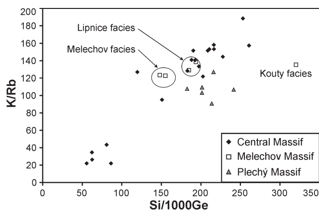
Fig. 3. Graph Si/1000Ge vs. K/Rb shows differences in geochemical evolution of individual magmatic centers within the South Bohemian Pluton.
