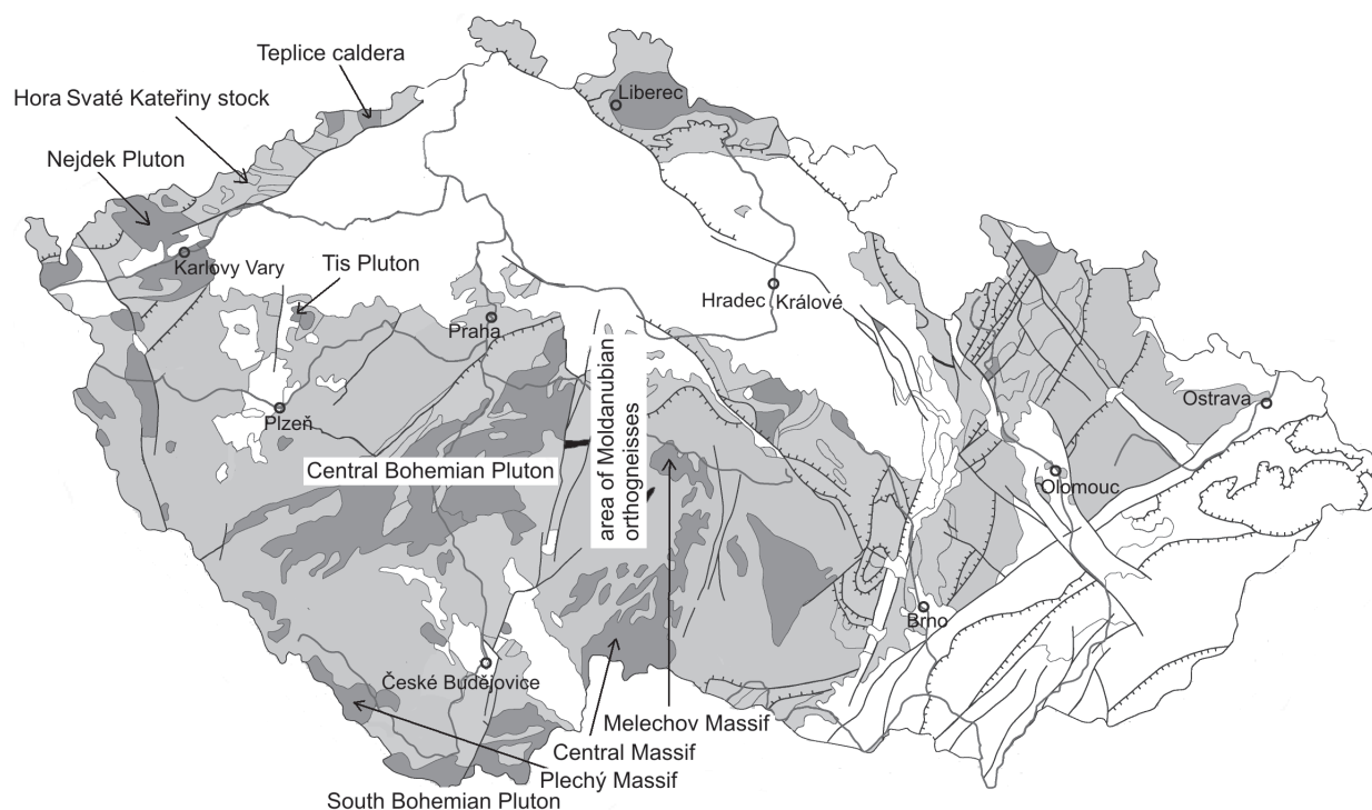
Fig. 1. Distribution of the studied granitic plutons within the Bohemian Massif, Czech Republic (from Cháb et al. 2010, modified). Black — orthogneiss, dark grey — granitoids, light grey — Variscan basement, white — post-Variscan sedimentary cover.
