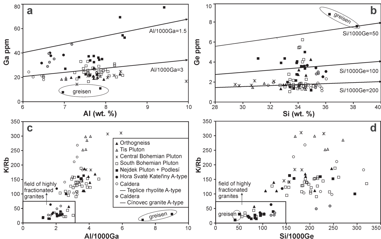
Fig. 2. a — Graph of Al vs. Ga. The highest Ga contents were detected in extremely fractionated facies of S-type granites in the western part of the Krušné Hory Mountains. The lowest contents of Ga were found in greisens. The contents of Al are slightly lower in A-type granitoids. The Al/Ga values are depicted in the right part of the graph. b — Graph of Si vs. Ge. The Ge content increases only slightly during the differentiation of plutons from 1–2 ppm to 4–5 ppm. The highest Ge contents were found in quartz-topaz greisens (7–9 ppm). The Si/Ge values are depicted in the right of the graph. c — Graph Al/1000Ga vs. K/Rb illustrates changes in the Al/Ga-ratio during evolution of individual plutons. d — Graph Si/1000Ge vs. K/Rb illustrates changes in the Si/Ge-ratio during evolution of individual plutons.
