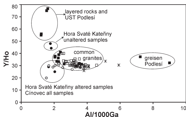
Fig. 5. Graph of \text{Al}/\text{Ga} versus \text{Y}/\text{Ho} ratios illustrates dissimilarity of various processes occurring in the late evolution of granites. See the text for explanation. For symbol descriptions, see Fig. 2.
