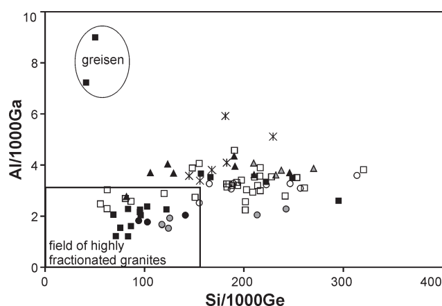
Fig. 4. Graph of Al/Ga versus Si/Ge ratios for comparison of evolution of both values. The Si/Ge ratio more accurately illustrates the general process of differentiation. Empirical field of highly fractionated granites with limits Si/1000Ge<150 and Al/1000Ga<3 is depicted. Greisens lie outside the magmatic trend. For symbol descriptions, see Fig. 2.
