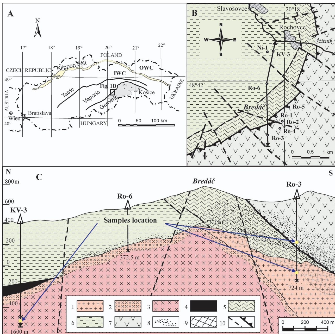
Fig. 1. A — Simplified tectonic-geological sketch of the Western Carpathians (Slovak part), displaying the principal tectonic units of the IWC and position of the study area. Explanations: OWC — Outer Western Carpathians, IWC — Inner Western Carpathians. B — Detailed geological sketch of the study area with the positions of principal exploration boreholes. Rocks symbols are identical as in Fig. 1C. C — Idealized geological profile across Rochovce granite body, with location of dated samples Ro-3/398.5 and Ro-3/676.6 m. Explanations: 1 — granite of the 2 nd intrusive phase, 2 — marginal fine-grained granite of the 1 st intrusive phase, 3 — coarse-grained porphyritic granite — 1 st phase, 4 — metagabbro, 5 — Rimava Formation, 6 — Slatviná Formation, 7 — Ochtná Formation, 8 — mineralized zone with sulphides and tungsten [W-zone], 9 — mineralized zone with molybdenite [Mo-zone], 10 — tectonic lines — fault and thrust.
