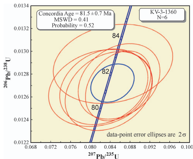
Fig. 4. SHRIMP U-Th-Pb zircon data of the Rochovce biotite granite (KV-3/1360 m sample).
