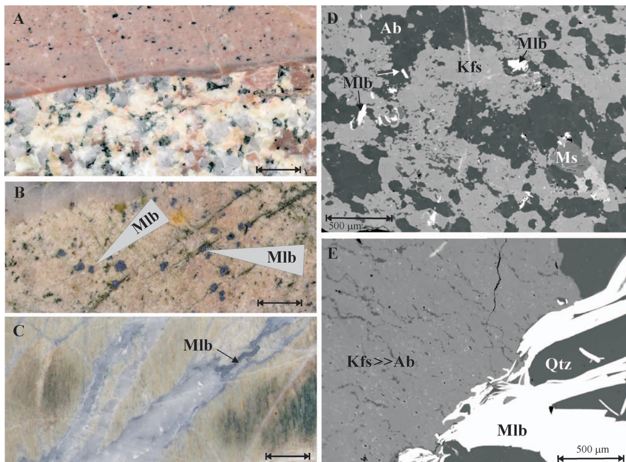
Fig. 2. A — Sharp contact of the narrow vein of fine-grained granite — 2 nd intrusive phase to coarse-grained granite of the 1 st phase with chilled margin. Sample taken from borehole KV-3 depth 1379.8 m. Scale bar 1 cm. B — Molybdenite-bearing (Mlb) veinlets structure in the fine-grained granite-porphyry of the 2 nd intrusive phase — sample Ro-3/676.6 m. Natural size (scale bar 1 cm). C — Quartz-molybdenite veinlet structure in host rock quartz phyllite of the Ochtiná Formation — sample Ro-3/398.5 m. Scale bar 1 cm. D — Tiny inclusions of molybdenite (Mlb) in medium-grained porphyry — sample Ro-2/532.3 m. Abbreviations: Ab — albite, Kfs — K-feldspar, Ms — muscovite. Back-scattered electron image (BSEI). E — Quartz-molybdenite (Qtz-Mlb) veinlet in phyllite rock (Ochtiná Formation); sample Ro-5/549.5 m; BSEI.
