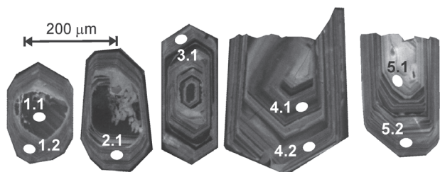
Fig. 3. Zircon CL images of the Rochovce granite sample KV-3/1360 m with location of the SHRIMP dating spots.
