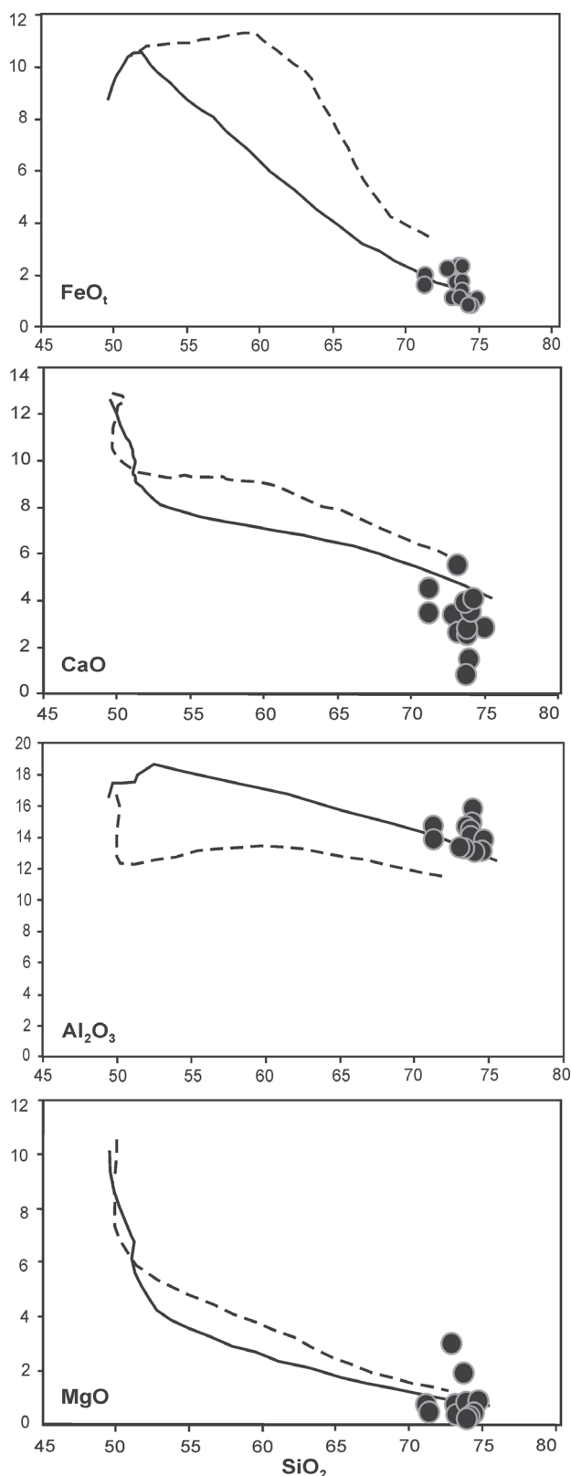
Fig. 10. \text{FeO}^T , \text{CaO} , \text{Al}_2\text{O}_3 and \text{MgO} vs. \text{SiO}_2 for Eldivan plagiogranites and MELTS (Ghiorso & Sack 1995) fractional crystallization modelling curves. Crystallization temperature interval is 1000–800 °C and f\text{O}_2 value is chosen as QFM + 1. Calculation parameters; 1 kbar hydrous (1 % \text{H}_2\text{O} ) (black continuous curve), 1 kbar anhydrous (0 % \text{H}_2\text{O} ) (black dashed curve).
