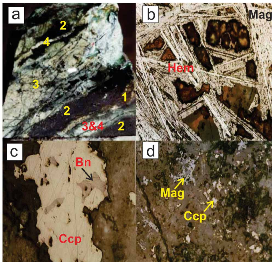
Fig. 6. a — shows intense and multiple replacement hand spacemen of skarn and formation of ore skarn. No. 1 — shows the remnant of brown garnet after replacement by magnetite. No. 2 — shows magnetite veins replacing garnet. No. 3 — shows an intense replacement of early rocks by sulfide and quartz. No. 4 — mineralized quartz veins belonging to the 4 th stage of alteration or hydrothermal activity; b — is a microphotograph of a polished section showing replacement of radial magnetite by hematite due to martitization. Blades consist of martite crystals (5–20 mm) which represent the hematitization of euhedral magnetite. The replacement process includes an initial iron atom diffusion through the oxygen framework leading to maghemite, followed by inversion of maghemite to hematite and development of distorted octahedrons; c — microphotograph of polished section shows replacement of magnetite and anhydrous minerals by patches of chalcopyrite along with bornite; d — microphotograph of polished section shows replacement of silicate minerals by magnetite and chalcopyrite.
