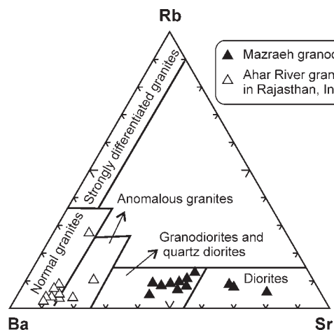
Fig. 10. a — Ternary diagram of Rb-Ba-Sr for igneous rocks of the Ahar Batholith in comparison with Ahar River granite from Rajasthan, India (after Thomas 1987); b — Plot of Nb vs. Zr for igneous rocks of the Ahar Batholith (after Wilson 1989).
