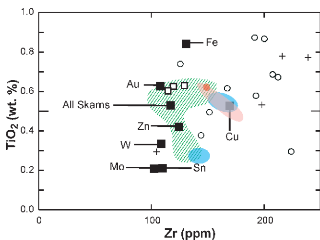
Fig. 11. Variation diagram of Zr vs. \text{TiO}_2 illustrating the relationship of igneous rocks of the Ahar Batholith associated with skarn deposit compared with other igneous rocks associated with skarn deposits. Plots of different skarns are produced after Meinert (1995) and Togla (2010).
