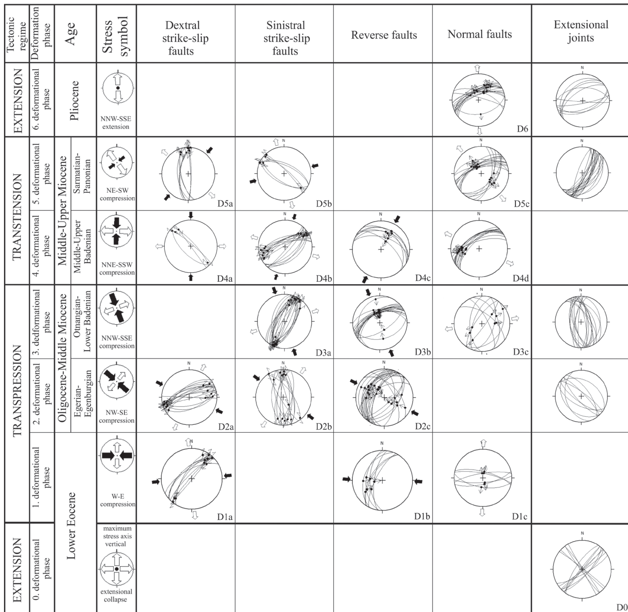
Fig. 6. Synoptic table of successive deformational phases D1 to D6 observed in all localities of the Súľov Mts. Each homogenous group of faults is presented by a stereogram (the fault planes are plotted as great circles with observed slip senses using stereographic projection — Schmidt net, lower hemisphere).
