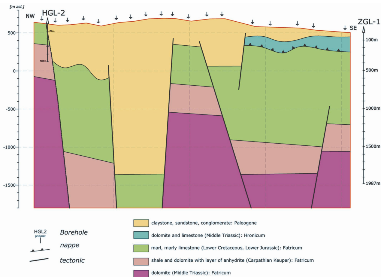
Fig. 4. Integrated geological-geophysical interpretation — geological section of the profile PF01.
