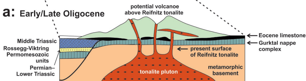
Fig. 9. Three-stage tectonic model for the evolution of the Wörthersee area in southeastern Austria. a — Time of intrusion of the Reifnitz tonalite with a potential volcano above it. b — Oligocene gentle folding and formation of antiforms and synforms. c — Formation of the peripheral bulge by flexuring the crust in front the North Karawanken thrust (after Nemes et al. 1997) and erosion of the Wörthersee antiform. White arrows indicate dominant vertical motion at the given time interval.
