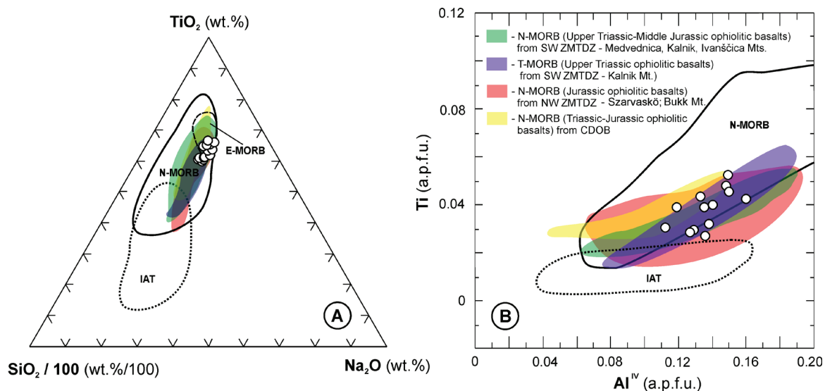
Fig. 14. Discriminant diagram \text{SiO}_2/100\text{--Na}_2\text{O--TiO}_2 (A) and \text{Al}^{\text{IV}}\text{--Ti} (B) (simplified after Beccaluva et al. 1989) for clinopyroxene from ortho-greenschists from Mt. Medvednica metamorphic complex. IAT=island-arc tholeiites, E-MORB=enriched mid-ocean ridge basalts, N-MORB=normal mid-ocean ridge basalts. Field of clinopyroxene composition of the Jurassic extrusives from the northeastern part of ZMTDZ (Szarvaskő complex in Mt. Bükk; Balla & Dobretsov 1984) and basalts from CDOB (Lugović et al. 1991) are plotted for correlation constraints.
