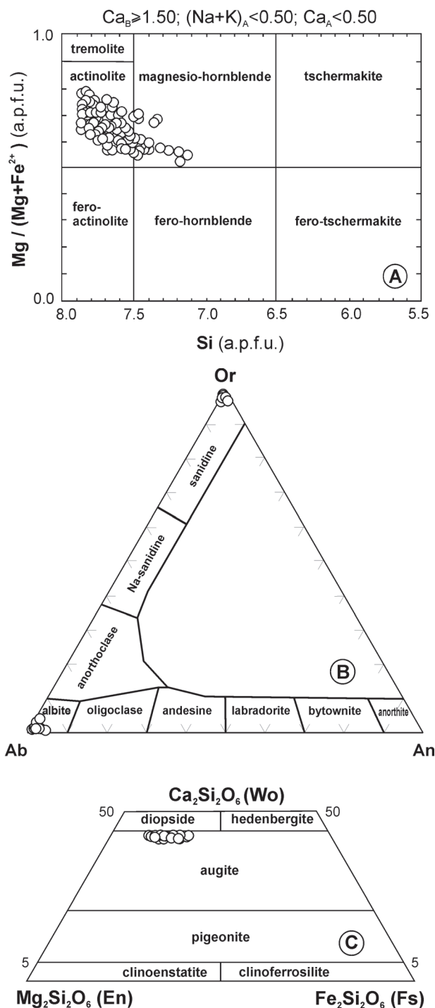
Fig. 6. Classification diagrams for: A — calcium amphibole [ \text{Si-Mg}/(\text{Mg}+\text{Fe}^{2+}) plot (Leake et al. 1997)], B — feldspar [ \text{Ab-An-Or} plot (Deer et al. 1992 and Dana et al. 1993)] C — clinopyroxene [ \text{En-Fs-Wo} ( \text{Mg}_2\text{Si}_2\text{O}_6\text{-Fe}_2\text{Si}_2\text{O}_6\text{-Ca}_2\text{Si}_2\text{O}_6 ) plot (Morimoto et al. 1998)], from ortho-greenschists from Mt. Medvednica metamorphic complex.
