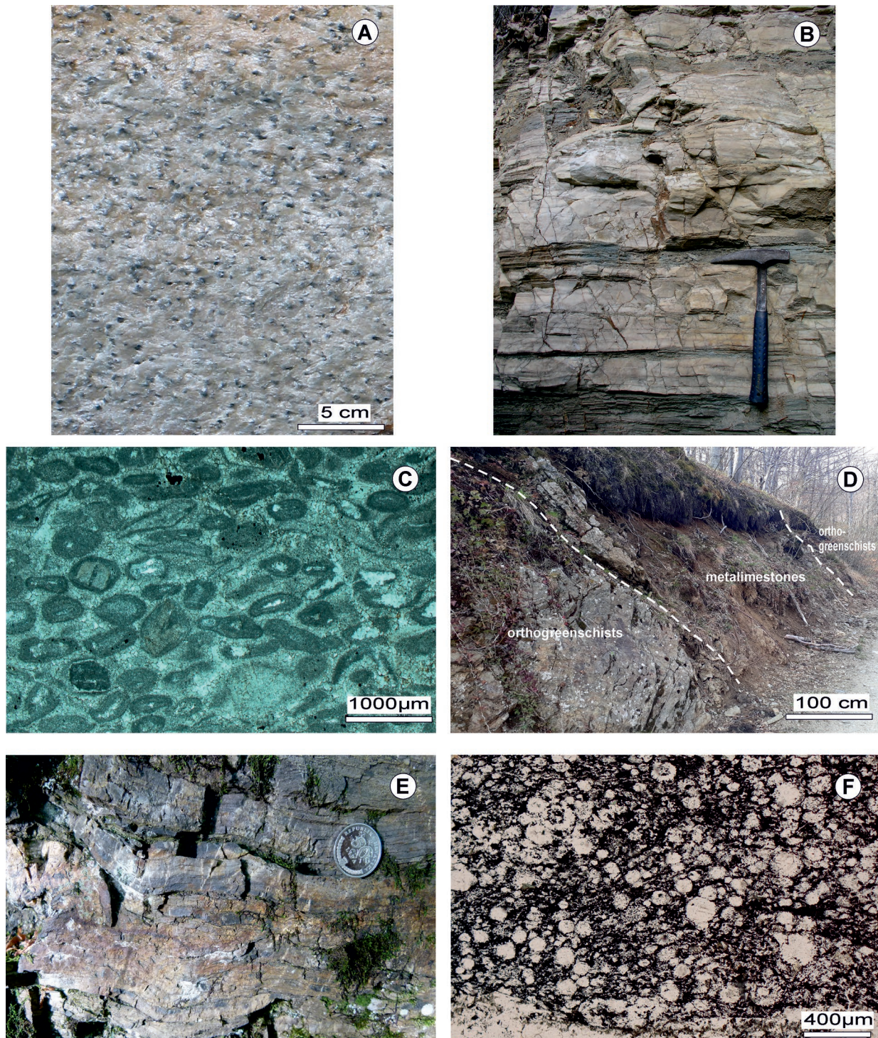
Fig. 3. Field occurrence of: A — chloritoid schists ( Stari Potok Unit ); B — marbles with greenschists interlayers ( Adolfovac Unit ); C — meta-limestones ooids ( Stari Potok Unit ); D — metalimestone interlayer (Anisian – Bithinian to Illyrian) in ortho-greenschists (metabazalts) ( Tusti Breg Unit ); E — metaradiolarites ( Mrzljak Unit ). Microphotograph of metaradiolarites ( F ) with recrystallized radiolarians in magnetite–hematite matrix ( Mrzljak Unit ).
