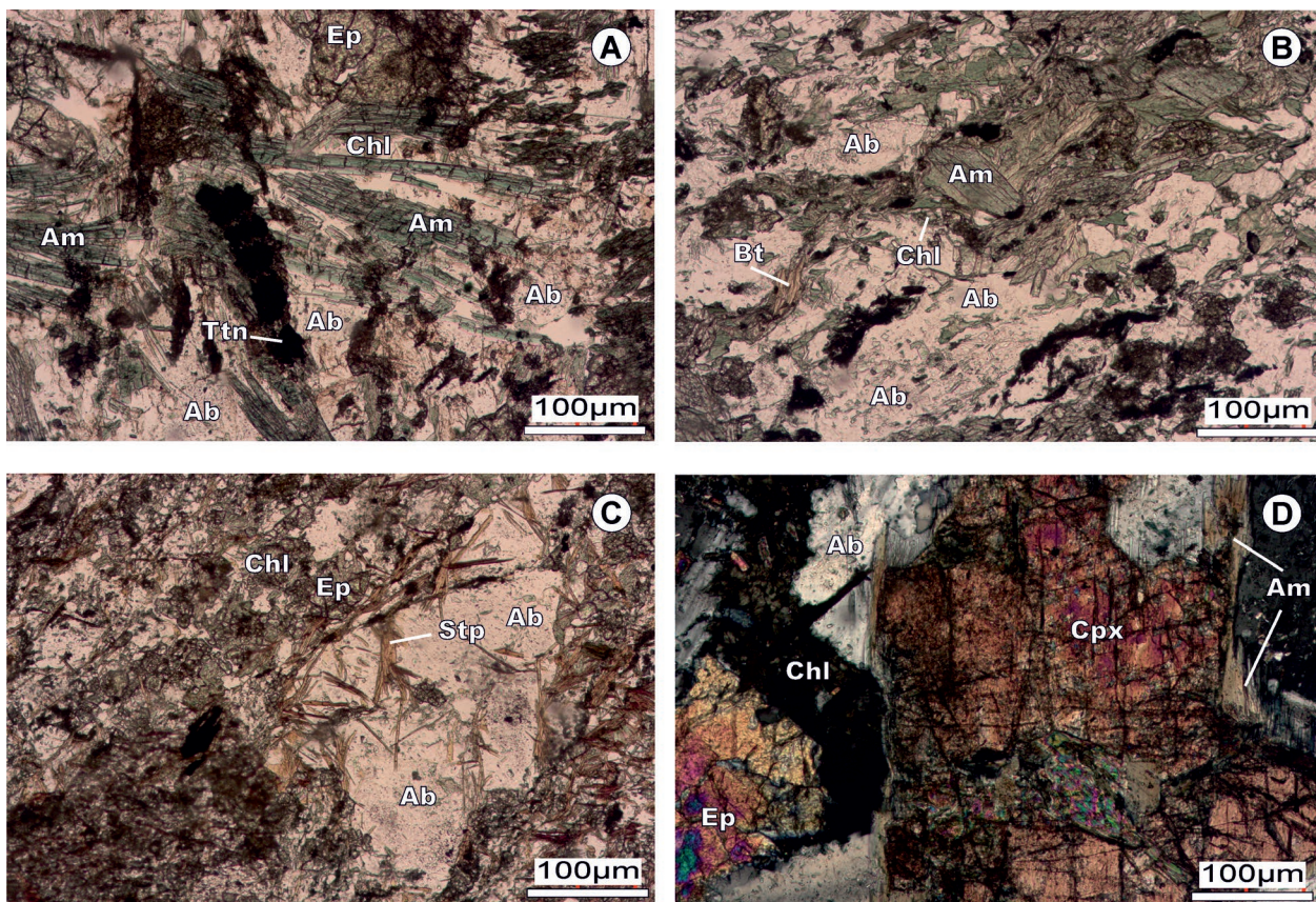
Fig. 5. Microphotographs of thin sections of: A — ortho-greenschist – metabasalt (N-), sample J-898 (epidote–amphibolite–greenschist facies; Sljeme Unit ); B — ortho-greenschist – metabasalt (N-), sample Zelj-23 (greenschist facies – middle parts; Sljeme Unit ); C — ortho-greenschist – metabasalt (N-), sample Run-1 (greenschist facies – lower parts; Sljeme Unit ); D — ortho-greenschist – metabasalt (N+), sample Md-4 (greenschist facies with relict of clinopyroxene; Tusti Breg Unit ). Mineral abbreviations after Kretz (1983): Ab=albite, Am=amphibole, Bt=biotite, Chl=chlorite, Cpx=clinopyroxene, Ep=epidote, Pl=plagioclase, Stp=stilpnomelane, Ttn=titanite.
