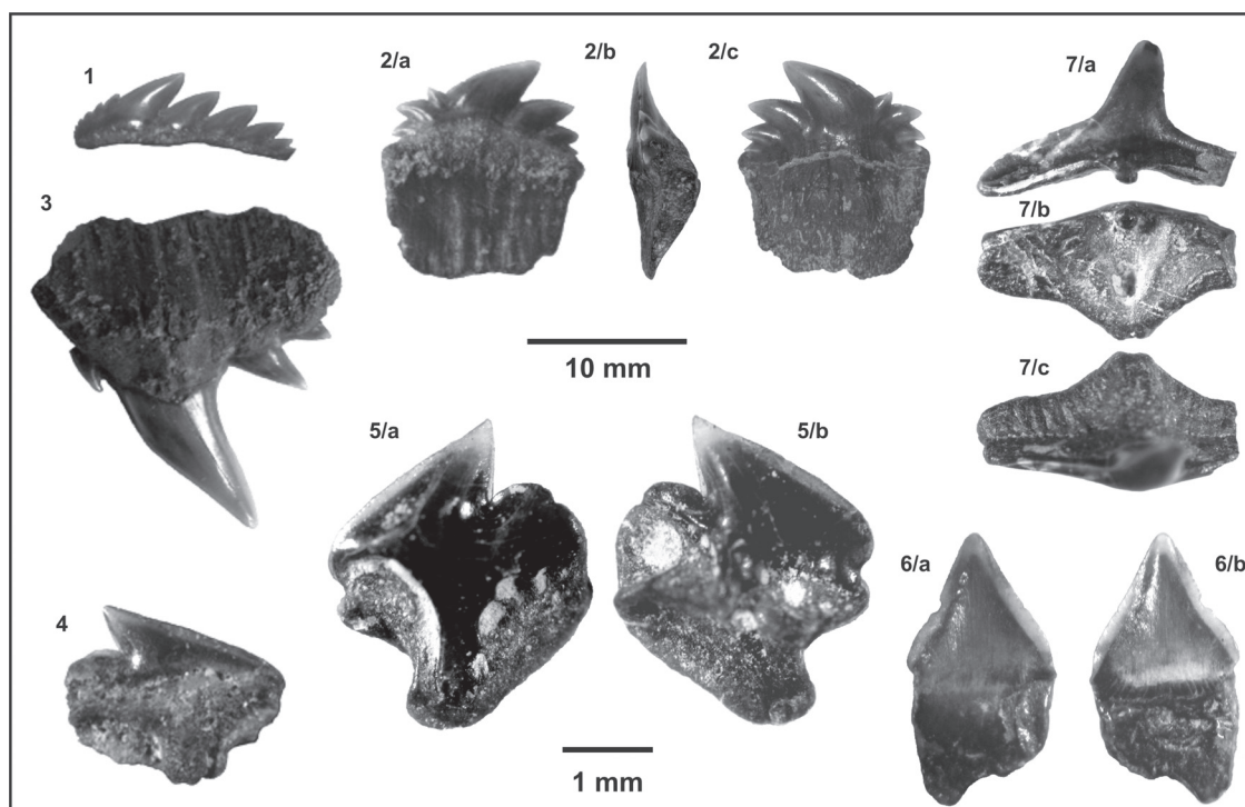
Fig. 3. 1–3 — Notorynchus primigenius : 1 — anterolateral (MÁFI-V14907); 2 — anterolateral (MÁFI-V14947), lin (a), mes (b), lab (c); 3 — medial (MÁFI-V14945). 4 — Squalus sp.: anterolateral (IT-M4-3), lab. 5 — Centrophorus sp.: anterolateral (IT-III-115), lab (a), lin (b). 6 — Isistius cf. triangulus : lower tooth (IT-M4-2), lab (a), lin (b) (scale bar: 1 mm). 7 — Squatina sp.: lateral (IT-M6-1/a), lab (a), bas (b) and oc (c). (1 mm scale for Figs. 3–6.)
