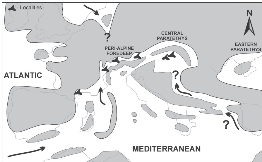
Fig. 7. Lower Miocene paleogeography (after Rögl 1998 modified at Rhine Graben after Kuhlemann & Kempf 2002). The shark teeth localities from west to east: Montpellier region, Swiss Molasse; Bavarian Molasse; Austria; Ipolytarnóc and Southern Slovakia.
