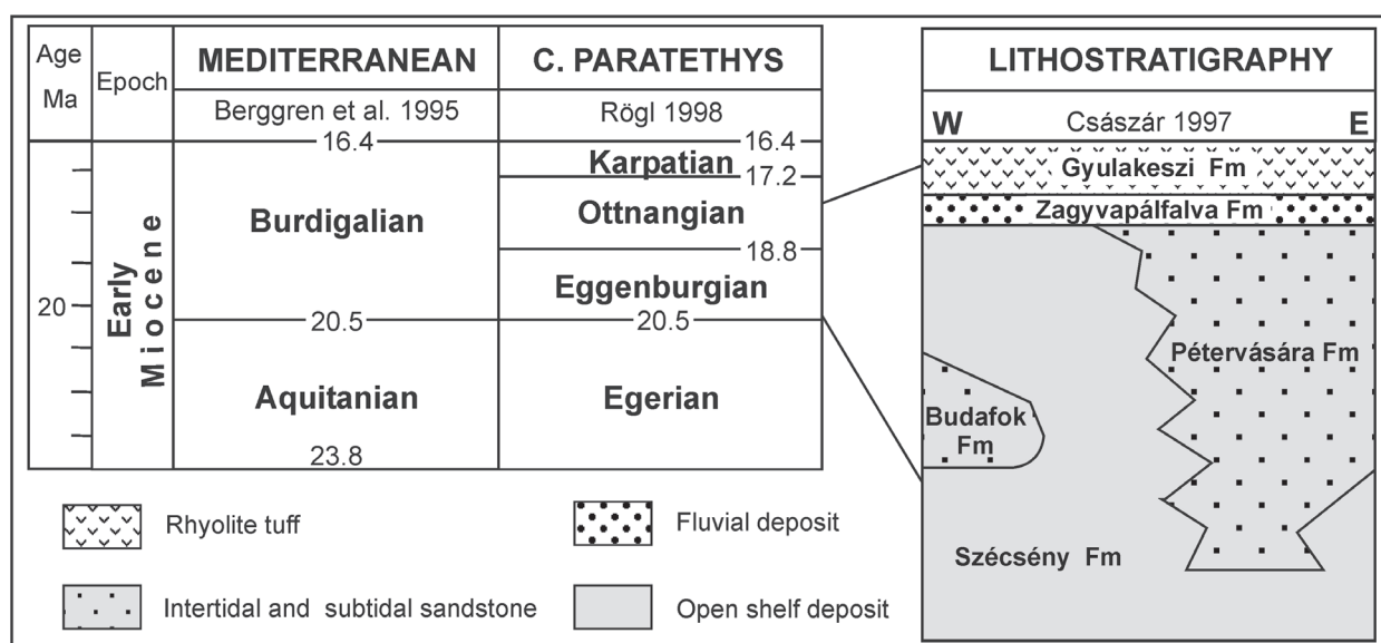
Fig. 2. Stratigraphic position of the Lower Miocene beds at Ipolytarnóc.
