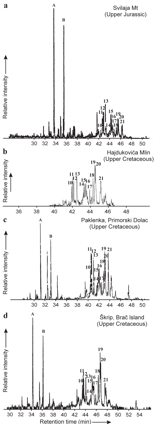
Fig. 7. Ion chromatograms showing the distribution of steranes ( m/z 217) in potential source rock (a,b) and oil seep (c,d) samples. Identification of the labeled compounds is given in Table 6.
