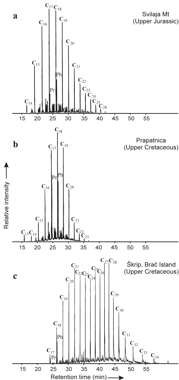
Fig. 5. Ion chromatograms showing the distribution of alkanes ( m/z 71) in potential source rock (a,b) and oil seep (c) samples. Peak identifications: C_x = n -alkanes with x carbon number; Pr = pristane; Ph = phytane.
