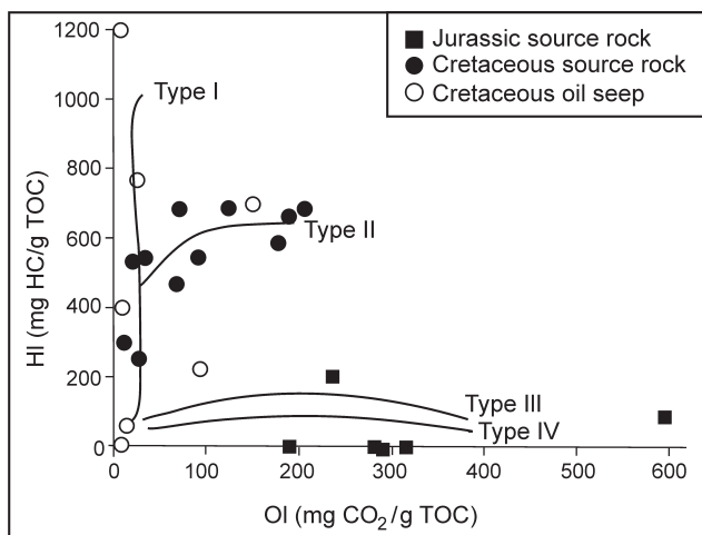
Fig. 3. Hydrogen index (HI) vs. oxygen index (OI) plot of the analysed samples.
