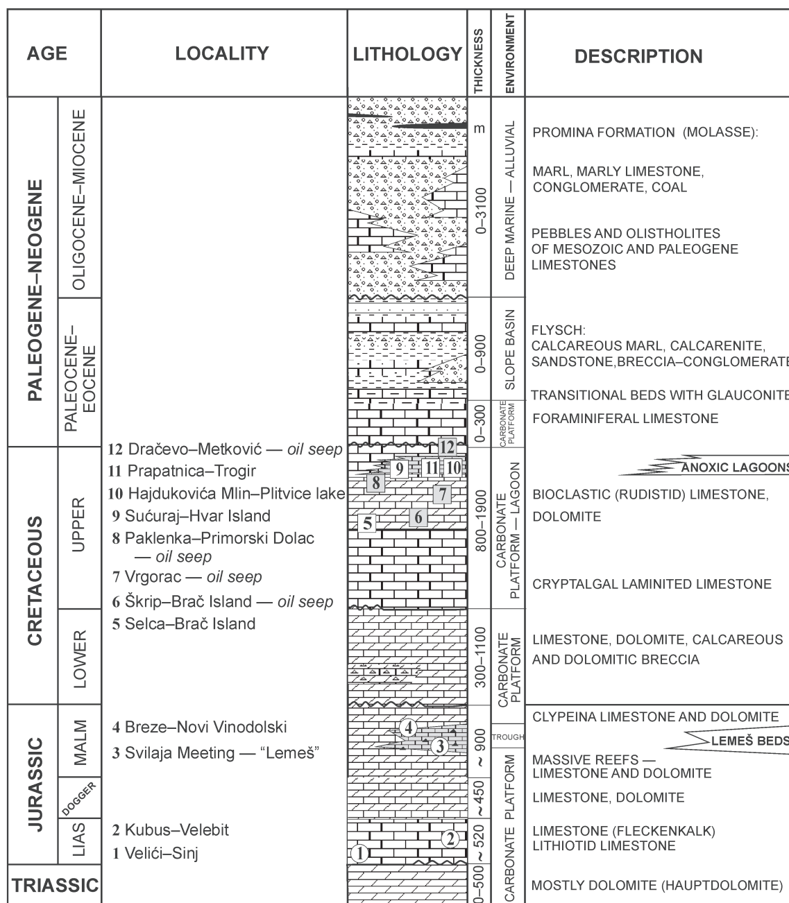
Fig. 2. Stratigraphic column of Cretaceous and Jurassic carbonate deposits in the Adriatic-Dinaric carbonate platform. (□ — Cretaceous potential source rock; ■ — Cretaceous oil seep; ○ — Jurassic potential source rock).
