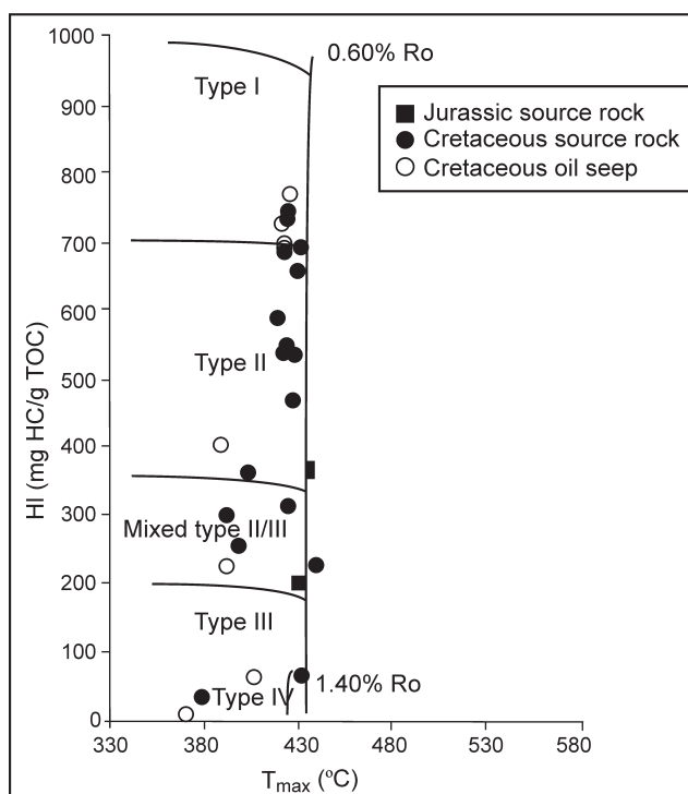
Fig. 4. Hydrogen index (HI) vs. T_{max} plot of the analysed samples.
