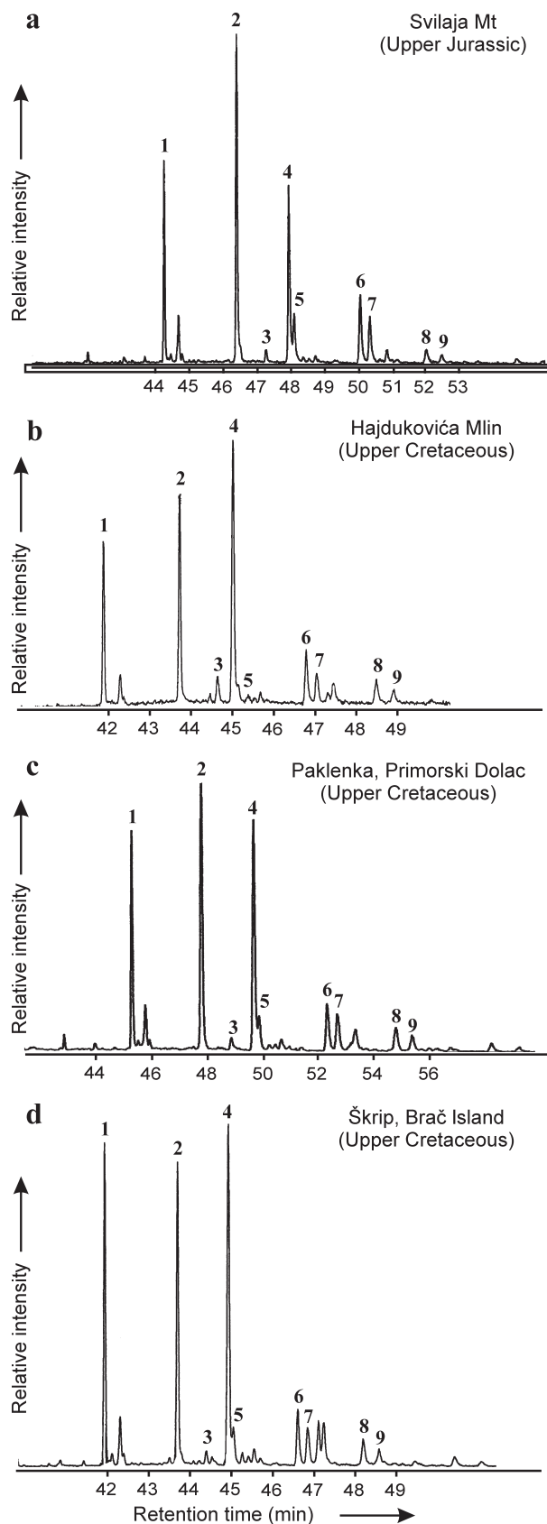
Fig. 6. Ion chromatograms showing the distribution of hopanes ( m/z 191) in potential source rock (a,b) and oil seep (c,d) samples. Identification of the labeled compounds is given in Table 6.
