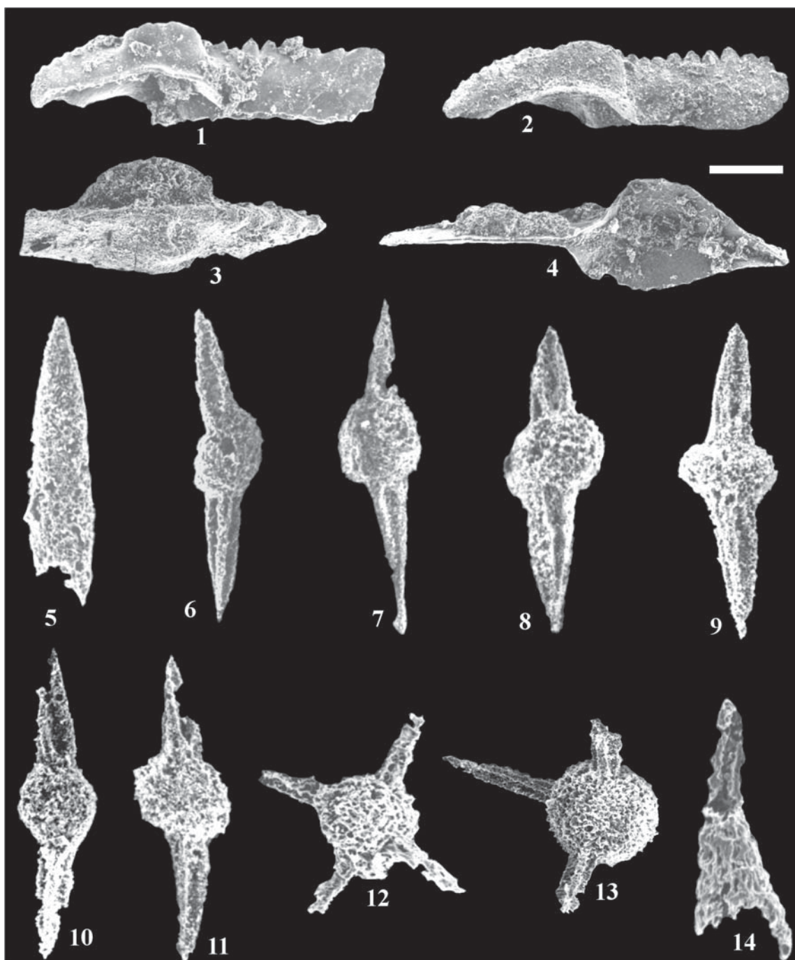
Fig. 12. Photomicrographs of the conodont and radiolarian faunas from the Cataloturan Nappe in Yahyali area. Figures 1–4 are from conodont fauna and figures 5–14 are from radiolarian faunas. 1–4 — Pa elements of Gnathodus pseudosemiglaber Thompson et Fellows. 1 is from sample 00CO11, 2–3 are from sample 00CO12 and 4 is from sample 00CO16, scale bar = 260, 280, 220 and 190 \mu\text{m} , respectively. 5 — Albaillella paradoxa group Deflandre, sample 00CO10, scale bar = 260 \mu\text{m} . 6–11 — Belowea variabilis Won, all specimens are from sample 00CO10, scale bar = 110, 105, 85, 95, 90 and 90 \mu\text{m} , respectively. 12–13 — Entactinia sp., both specimens are from sample 00CO10, scale bar = 90 and 120 \mu\text{m} . 14 — Archocyrtium sp. Sample 00CO6, scale bar = 70 \mu\text{m} .
