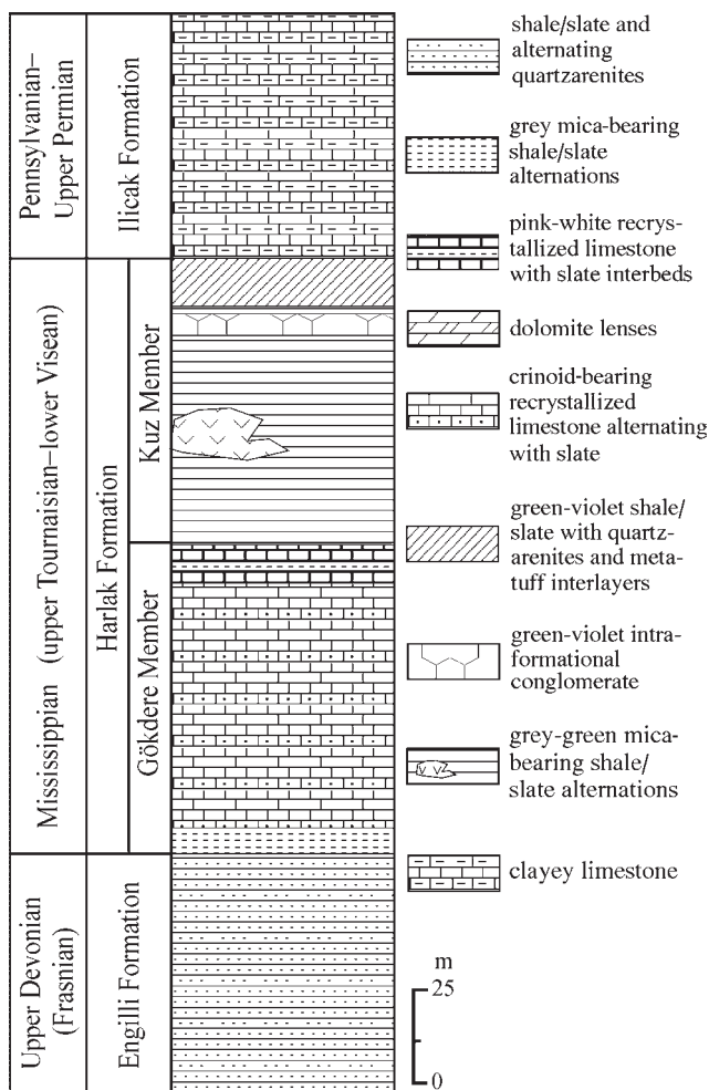
Fig. 3. Generalized columnar section of the Sultan Dağı Unit in Harlak village (Akşehir). (Modified from Özgül et al. 1991a.)
