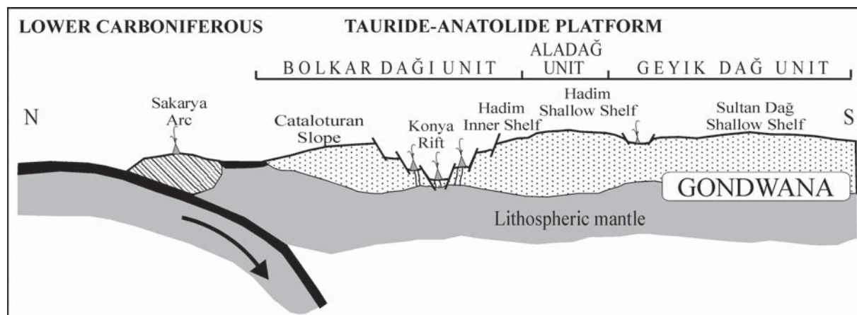
Fig. 13. Schematic reconstruction of the Tauride-Anatolide Platform for Mississippian.
