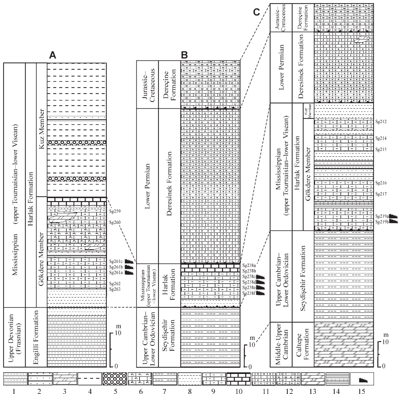
Fig. 4. Measured section of A — Harlak Formation near Akşehir, B — The Gökdere Member in old Deresinek village, C — The Gökdere Member in Eberdere village. 1 — pink-white, grey, brown quartzarenites; 2 — metasandstone lenses; 3 — dolomite lenses; 4 — grey-violet, green shales/slates; 5 — grey-green intra-formational pebblestone; 6 — grey, crinoid-bearing laminated, recrystallized limestone; 7 — green mica-bearing shales/slates; 8 — green shales/slates; 9 — grey-black laminated, recrystallized limestone with calcschist interlayers; 10 — pink-white-grey recrystallized limestone; 11 — grey-black-grey crinoid-bearing recrystallized limestone with calcschist interlayers; 12 — grey-black-grey cherty, recrystallized limestone; 13 — reddish-black-brown dolomite, dolomitic limestone; 14 — green-grey quartzarenites-bearing slate, 15 — conodont localities.
