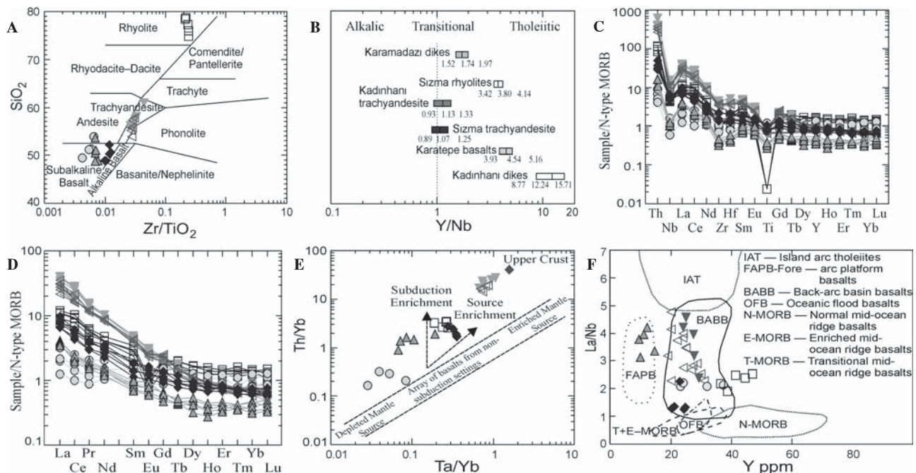
Fig. 8. A — Classification of the metamagmatic rocks of the Halıcı Group. B — Y/Nb discrimination diagrams of Pearce & Cann (1973). C,D — N-MORB normalized multivariation and REE diagrams (normalization values from Sun & McDonough 1989); Tectonic discrimination diagrams of metamagmatic rocks of Halıcı Group. E — Th/Yb-Ta/Yb diagram (Pearce 1983). F — La/Nb-Y diagram (Floyd et al. 1991). Closed circle — metadiabase dikes near the Kadınhanı area, closed triangle — Karatepe basalts, closed diamond — Karamadazi Dağı metadiabase dikes (near Yahyali), open triangle — trachyandesite in Kadınhanı village, reversed closed triangle — trachyandesite in Sızma village, open square — metarhyolite in Talas creek near Yükselen village.
