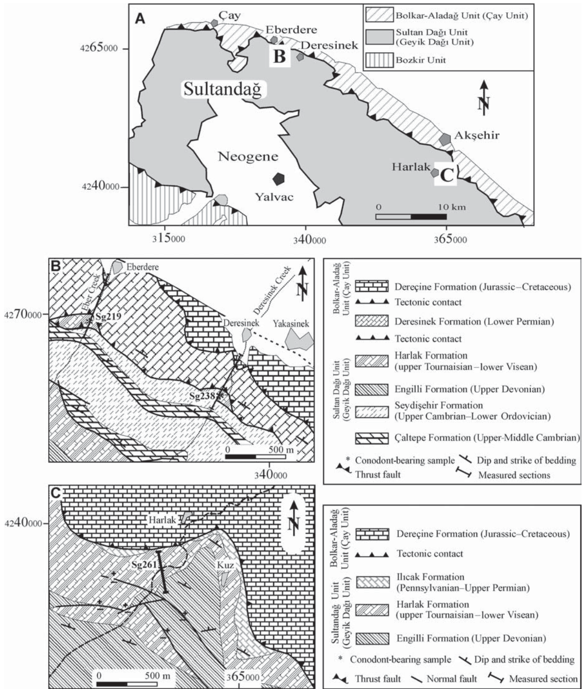
Fig. 2. A — Structural map of Sultan Dağı area. Geological map of B — Deresinek and Eberdere area (Çay), C — Harlak (Akşehir) area (modified from Özgül et al. 1991a).
