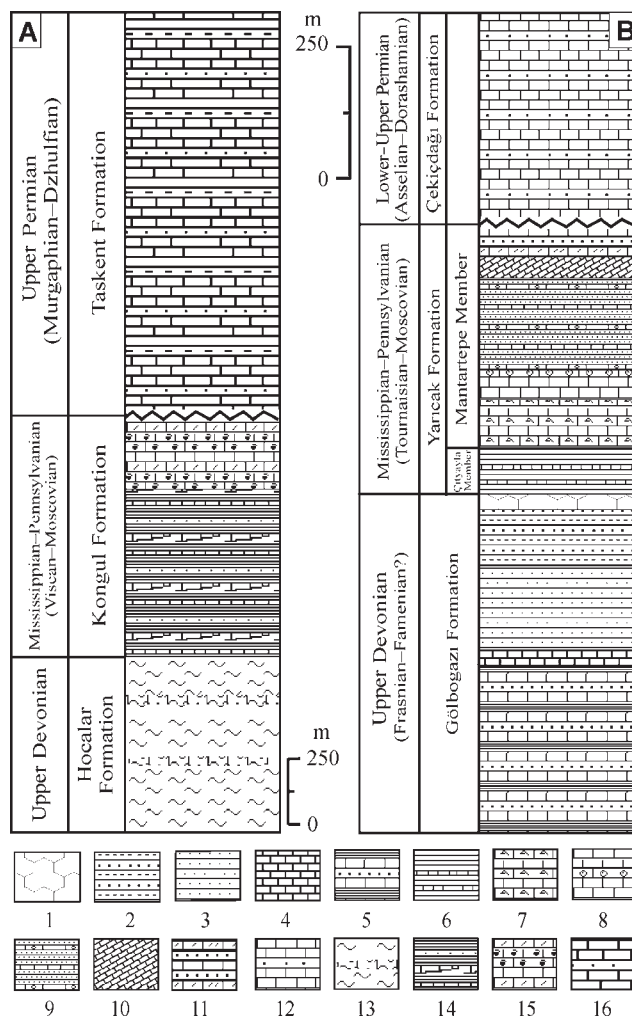
Fig. 9. Generalized columnar section of A — The Kongul Formation of the Bolkar Dağı Unit, B — Yarıcağ Formation of the Aladağ Unit in the Hadim area. 1 — conglomerate; 2 — quartzarenite-shale alternation; 3 — quartzarenites; 4 — limestone; 5 — limestone, shale and sandstone alternation; 6 — shale with sandy limestone interlayers; 7 — limestone with gastropods, crinoids and algae; 8 — oolitic limestone with quartzarenite interlayers; 9 — quartzarenites with foraminifers-bearing limestone interlayers; 10 — foraminifers and algae-bearing limestone; 11 — quartzarenite-limestone alternations; 12 — limestone-clayey limestone-shale alternation with quartzarenite interlayers; 13 — slate-quartzarenite recrystallized limestone alternation; 14 — shale-limestone alternation; 15 — crinoid-, brachiopod-, foraminifers-bearing oolitic limestone with rare shale interlayers; 16 — foraminifers-, algae-bearing limestone with rare quartzarenites and shale interlayers. (After Özgül 1997.)
