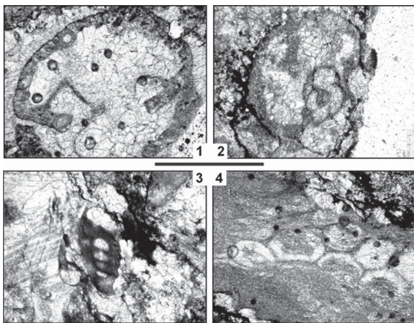
Fig. 7. Characteristic foraminifers and algae from the Mississippian Halıcı Group (Sample KC-16) in the Bolkar Dağı Unit in the Konya area. Scale bar represent 0.5 mm. All specimens are from sample C-16. 1 — Bradyina ex gr. rotula (D'Eichwald), subaxial section. 2 — Cribrospira ex gr. panderi (von Moeller), sagittal section. 3 — Eostaffella ex gr. mosquensis Vissarionova, axial section. 4 — Koninckopora ex gr. inflata (de Koninck), oblique section.
