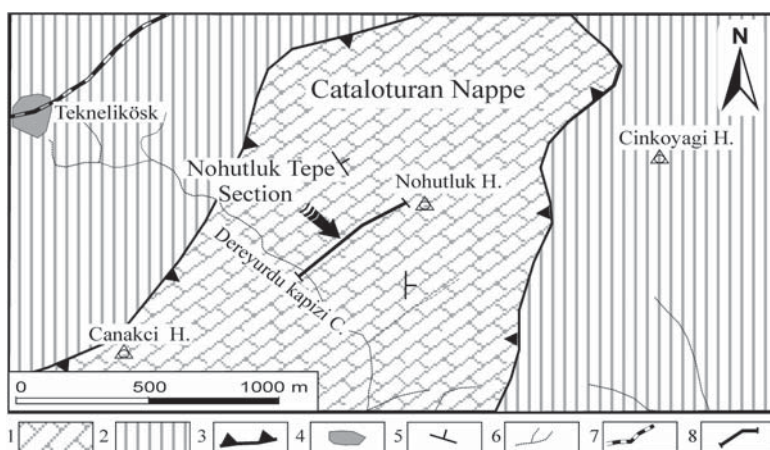
Fig. 10. Geological map of the area around Nohutluk Tepe section in Cataloturan Nappe. 1 — Carboniferous rock units; 2 — Senonian ophiolitic melange; 3 — thrust fault; 4 — settlement; 5 — dip and strike of bedding; 6 — drainage systems; 7 — main roads; 8 — location of the Nohutluk Tepe section. (Modified from Aksay 1980.)
