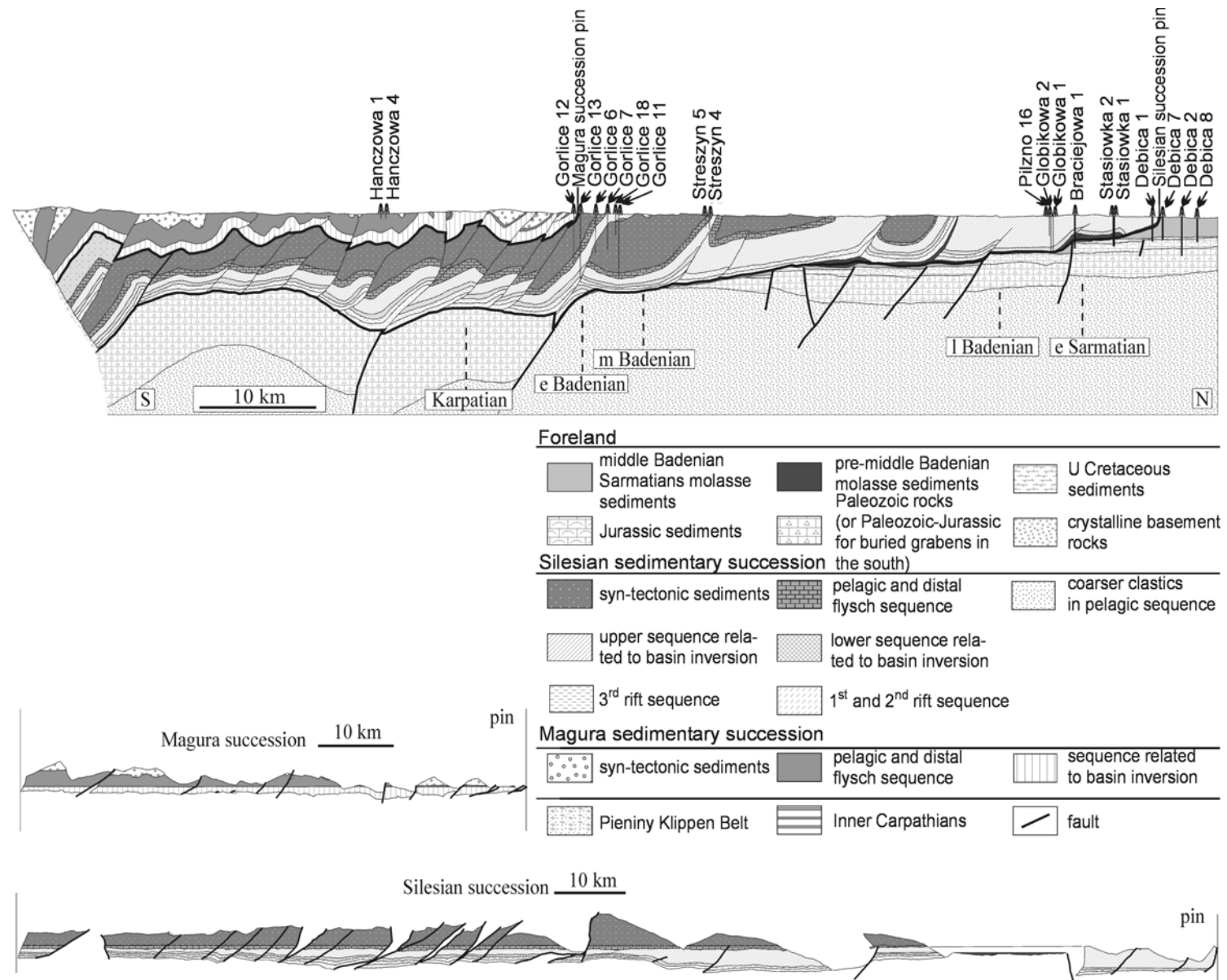
Fig. 4. A balanced and restored cross-section No. 3. The thick dashed vertical line indicates the southernmost extent of autochthonous molasse sediments of an indicated age, located below the accretionary wedge and inferred from well penetrations in the broader area. The layers of the Magura and Silesian sedimentary section are those introduced in Fig. 2 as a result of grouping facies. Molasse sediments are divided into groups of pre-middle Badenian and middle Badenian-Sarmatian. The vertical scale equals the horizontal scale.
