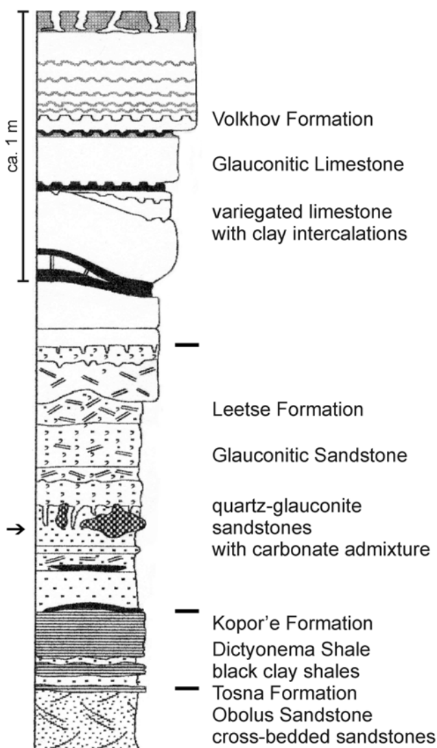
Fig. 2. Schematic drawing of the geological profile at the right bank of the Tosna River, ca. 200 m N of the Sablino Waterfall. The layer rich in phosphatized burrows is marked by arrow.
