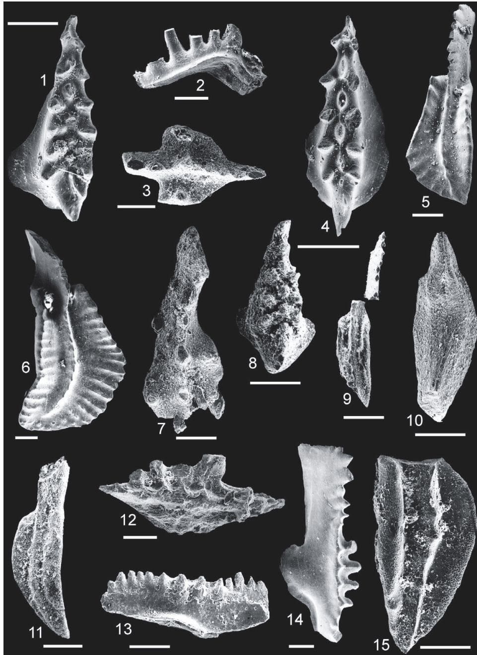
Fig. 7. Representative conodonts from the Saimbeyli-Tufanbeyli area, Eastern Taurides. The position of the samples is indicated in Figs. 5–8. The samples are deposited in the Geology Department of the General Directorate of Mineral Research and Exploration (MTA), Ankara. 1, 4 — Icriodus cf. brevis Stauffer, Pa element, upper view, sample CON-37, uppermost part of the Safak Tepe Formation, upper Givetian; 1 — rep.-no. 27-11/III-46; 4 — rep.-no. 27-11/III-44. 2 — Oulodus ? sp., Pb element, sample CON-37 (see Fig. 6), upper Givetian, rep.-no. 27-11/III-50. 3 — Ancyrodella pristina Khalimbadza et Chernyseva, Pa element, upper view, sample CON-21, upper reefal limestone member of lower Gümüşali Formation, lower Frasnian, rep.-no. 27-11/III-56. 5–6 — Polygnathus cf. parawebbi Chatterton; Pa element, upper view, sample CON-37 (see Fig. 6), upper Givetian; 5 — rep.-no. 27-11/III-43; 6 — rep.-no. 27-11/III-42. 7–8 — Icriodus brevis Stauffer, sample CON-20, lower reefal limestone member of lower Gümüşali Formation (see Fig. 8), lower Frasnian; 7 — broken Pa element, upper view, rep.-no. 27-11/III-41; 8 — Pa element, upper view, rep.-no. 27-11/III-54. 9–11 — Polygnathus xylus Stauffer, sample CON-21, upper reefal limestone of lower Gümüşali Formation, lower Frasnian; 9 — Pa element, free blade broken during preparation for SEM, upper view, rep.-no. 27-11/III-57; 10 — Pa element, lower view, rep.-no. 27-11/III-55; 11 — upper view, rep.-no. 27-11/III-59. 12 — Pseudopolygnathus vogesi Rhodes, Austin et Druce, Pa element, upper view, sample CON-23, lowermost Naltaş Member of basal Ziyarettepe Formation, uppermost Famennian, rep.-no. 27-11/III-2. 13–14 — Bispathodus aculeatus aculeatus (Branson et Mehl), Pa element, sample CON-23 (see Fig. 8), uppermost Famennian; 13 — lateral view, rep.-no. 27-11/III-1; 14 — oblique upper view, rep.-no. 27-11/III-4. 15 — Polygnathus cf. communis Branson et Mehl, sample CON-18, uppermost part of Naltaş Member, lower Ziyarettepe Formation, uppermost Famennian, rep.-no. 27-11/III-40. All scale bars = 100 µm.
