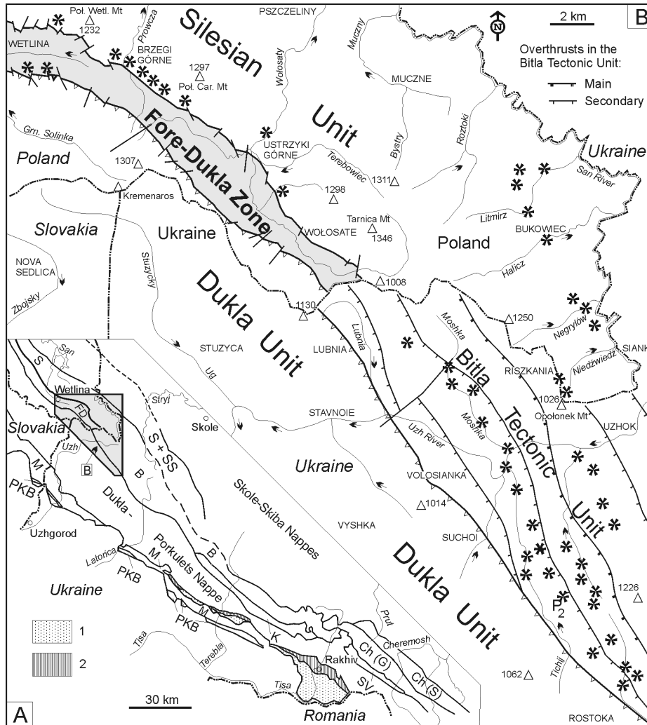
Fig. 9. A: Fore-Dukla Zone against a background of the main tectonic elements of the Eastern Carpathians (after Żytko 1999; simplified); emphasized the location of recent position of the Maramureș Massif and Rakhiv-Ceahlău Nappe — the area with rocks similar to the studied exotics: 1 — Maramureș Massif and their post-Austrian covers, 2 — Rakhiv-Ceahlău Nappe; B — Bitla tectonic unit, Ch (G) — Chornogora Nappe (Goverla), Ch (S) — Chornogora Nappe (Skupovna), FD — Fore-Dukla Zone, K — Krasnoshora Subunit, M — Magura Nappe, PKB — Pieniny Klippen Belt, S — Silesian Nappe, S + SS — Silesian Nappe (northern part) and Sub-Silesian Nappe, SV — Svidovets tectonic subunit. B: Exotic occurrences (stars) in the most southern part of the Silesian Nappe and the Bitla tectonic unit, the Bieszczady Mts (boundaries of the Fore-Dukla Zone after Haczewski et al. (submitted a,c); overthrusts in the Bitla tectonic unit after Glushko et al. (1999); exotic localities — see in the text).
