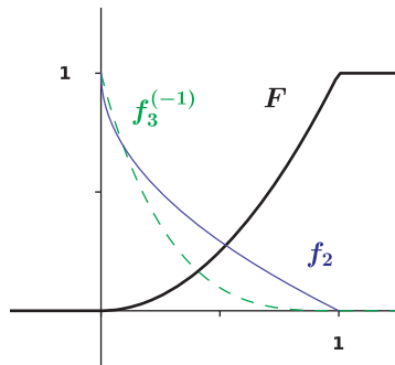
FIGURE 4. Illustration of Example 3 with non-invertible case n = 3 .
