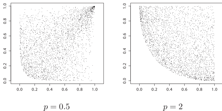
FIGURE 5. Sampling from copula family constructed in Example 4.
