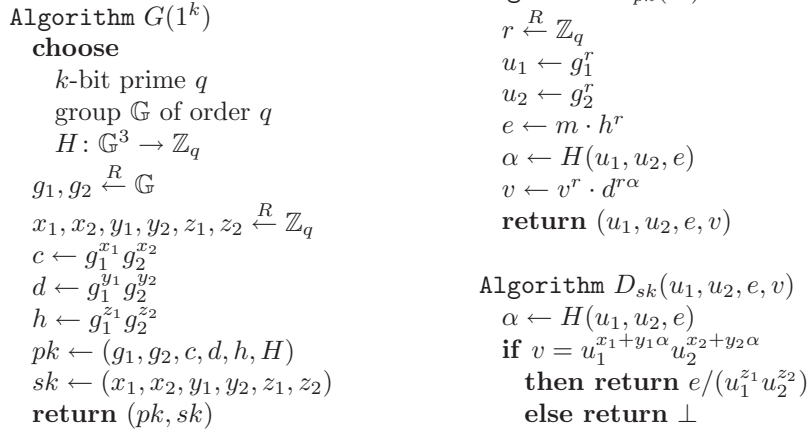
FIGURE 3. The Cramer-Shoup encryption scheme.
