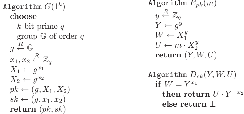
FIGURE 1. The DEG encryption scheme.
