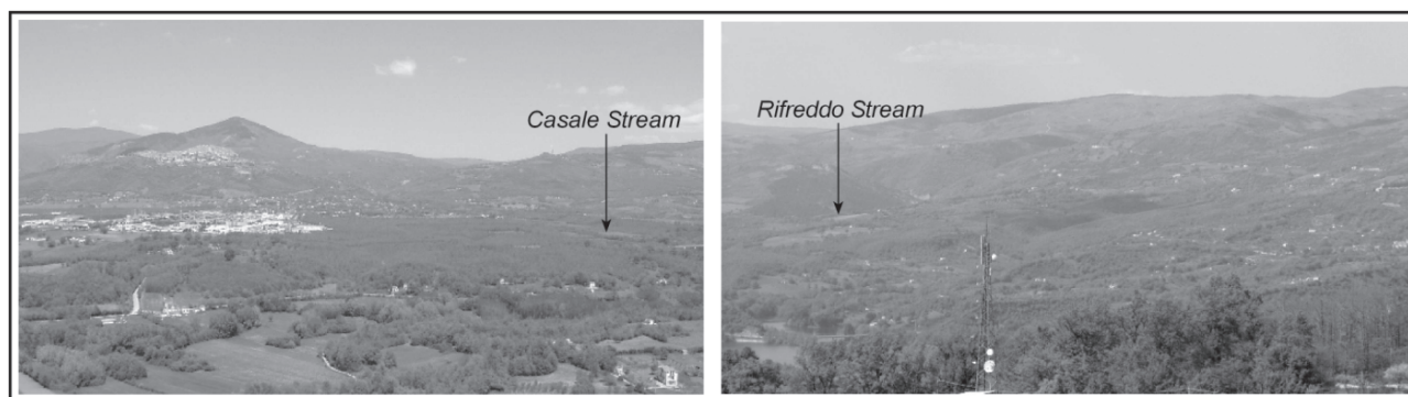
Fig. 6. Fan surfaces and vertical incision of the Casale (a) and Rifreddo (b) Streams.
