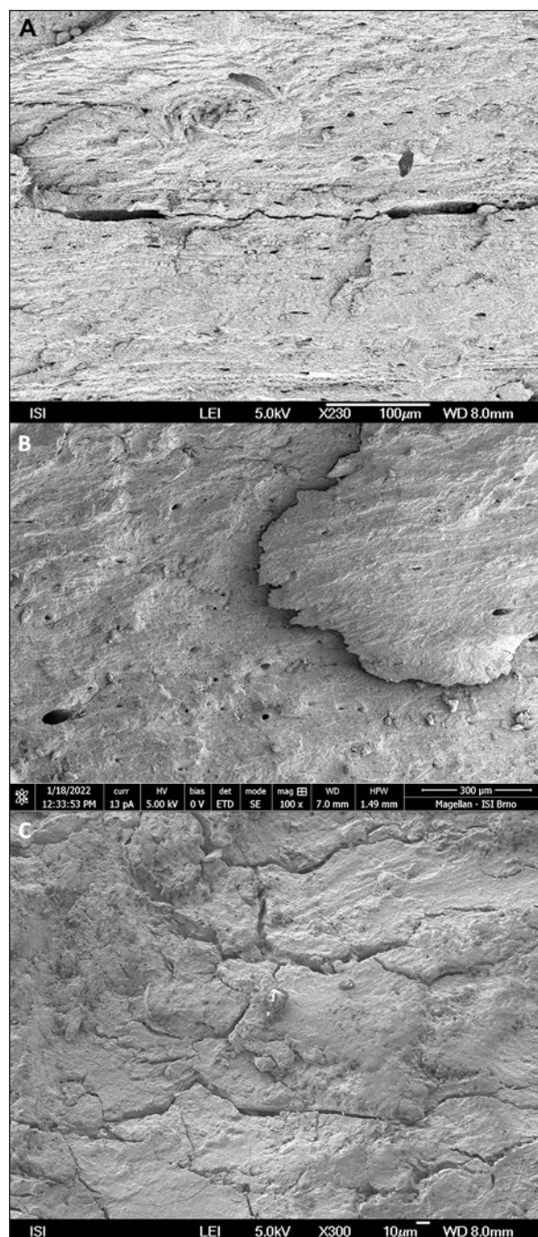
Fig. 4. Types of micro-cracking mostly observed by SEM. A – longitudinal cracking connecting two Haversian canals (sample C, magnification 230×); B – micro-crack lining the plate-like- surface protrusion (sample Q, magnification 100×); C – irregular reticulate micro-cracking observed in frozen samples (sample D, magnification 300×). Photo Z. Pokorná and S. Boriová.
