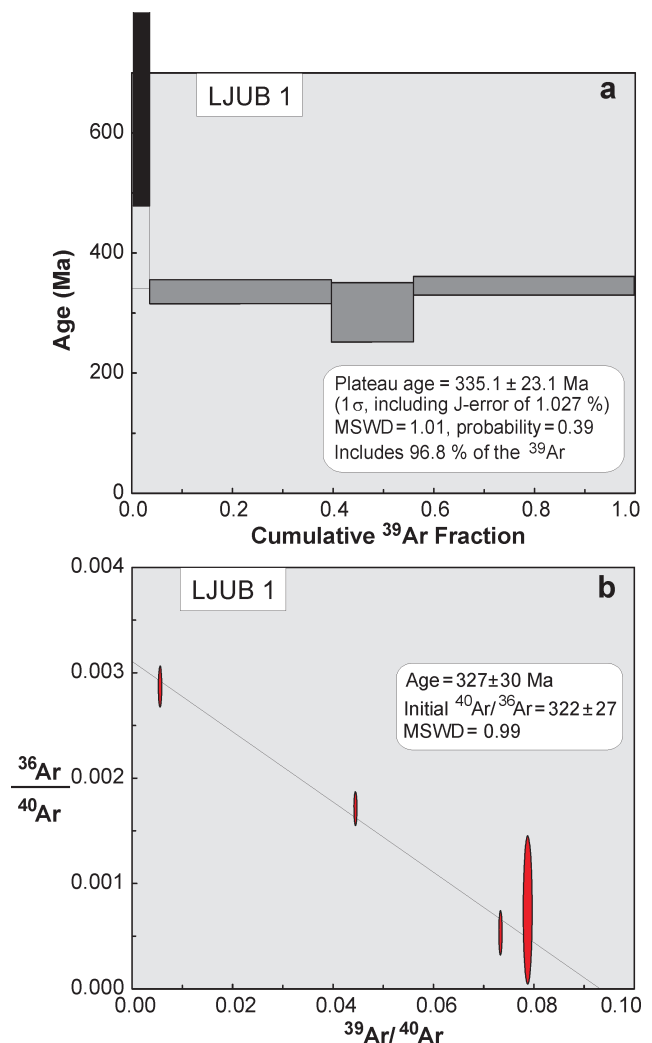
Fig. 6. ^{40}\text{Ar}/^{39}\text{Ar} apparent age spectra and inverse isochrone of the white mica (ca. 10–20 grains for each sample) from phyllite of the Ljubija open pit (Paleozoic Sana-Una Unit). Laser energy increases from left to right. Vertical width of bars represents 1 \sigma error. Steps used for calculation of plateau ages are delineated by bar.
