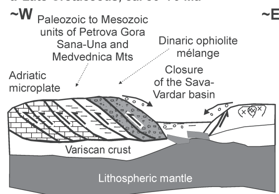
Fig. 7. Simplified tectonic models for the tectonic evolution of northwestern Dinarides.
